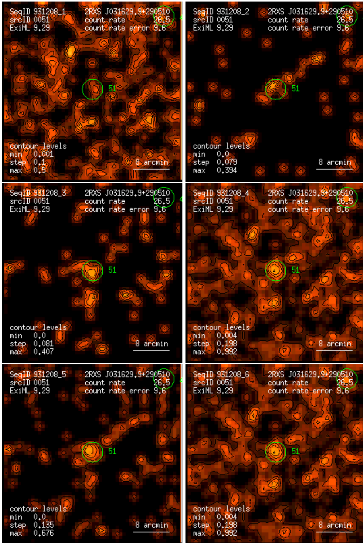
Figure 51: RASS 931208: detection 0051: band rate images, Gaussian filter: (1) PSPC channels 11 – 41, (2) 52 – 90, (3) 91 – 201, (4) 11 – 235, (5) 52 – 201, (6) 11 – 201. Broad band rates in counts/ks. Band rate contour levels in counts/ks/arcmin 2 .
