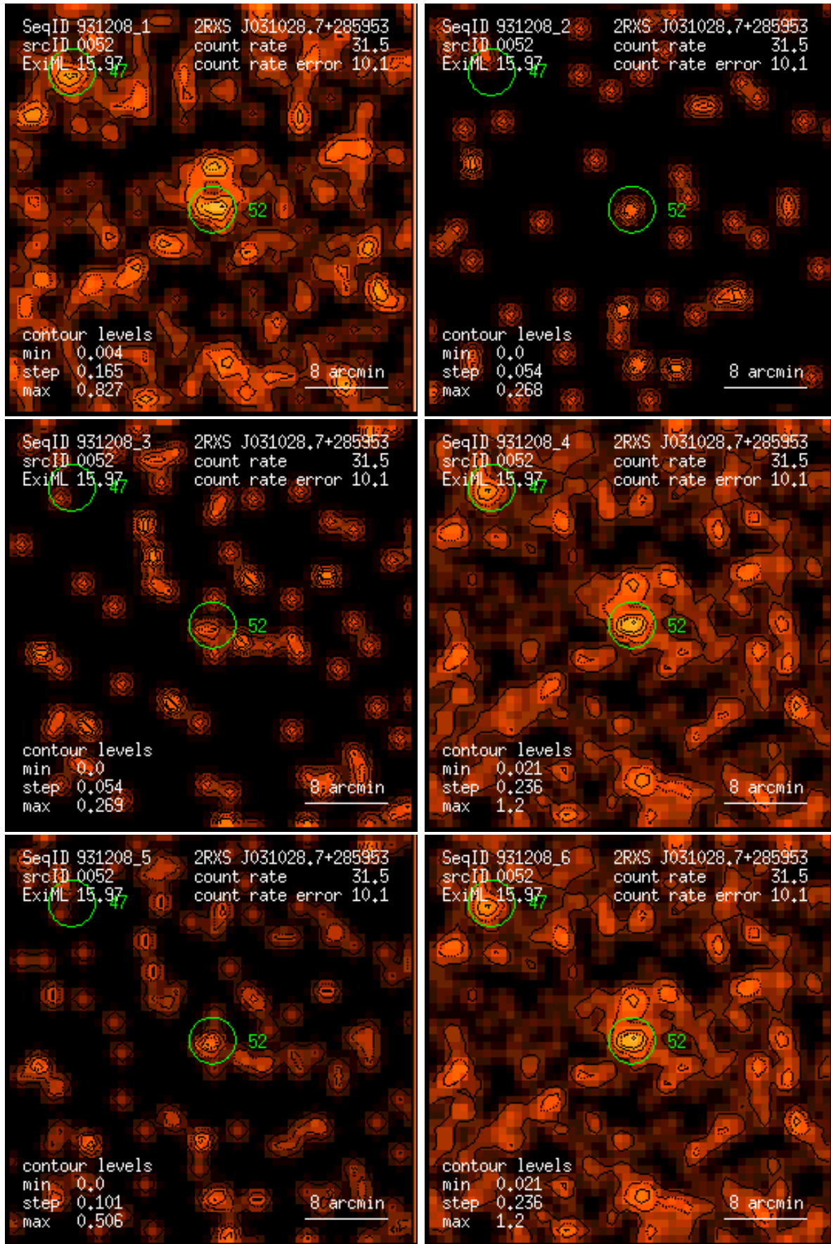
Figure 52: RASS 931208: detection 0052: band rate images, Gaussian filter: (1) PSPC channels 11 – 41, (2) 52 – 90, (3) 91 – 201, (4) 11 – 235, (5) 52 – 201, (6) 11 – 201. Broad band rates in counts/ks. Band rate contour levels in counts/ks/arcmin 2 .
