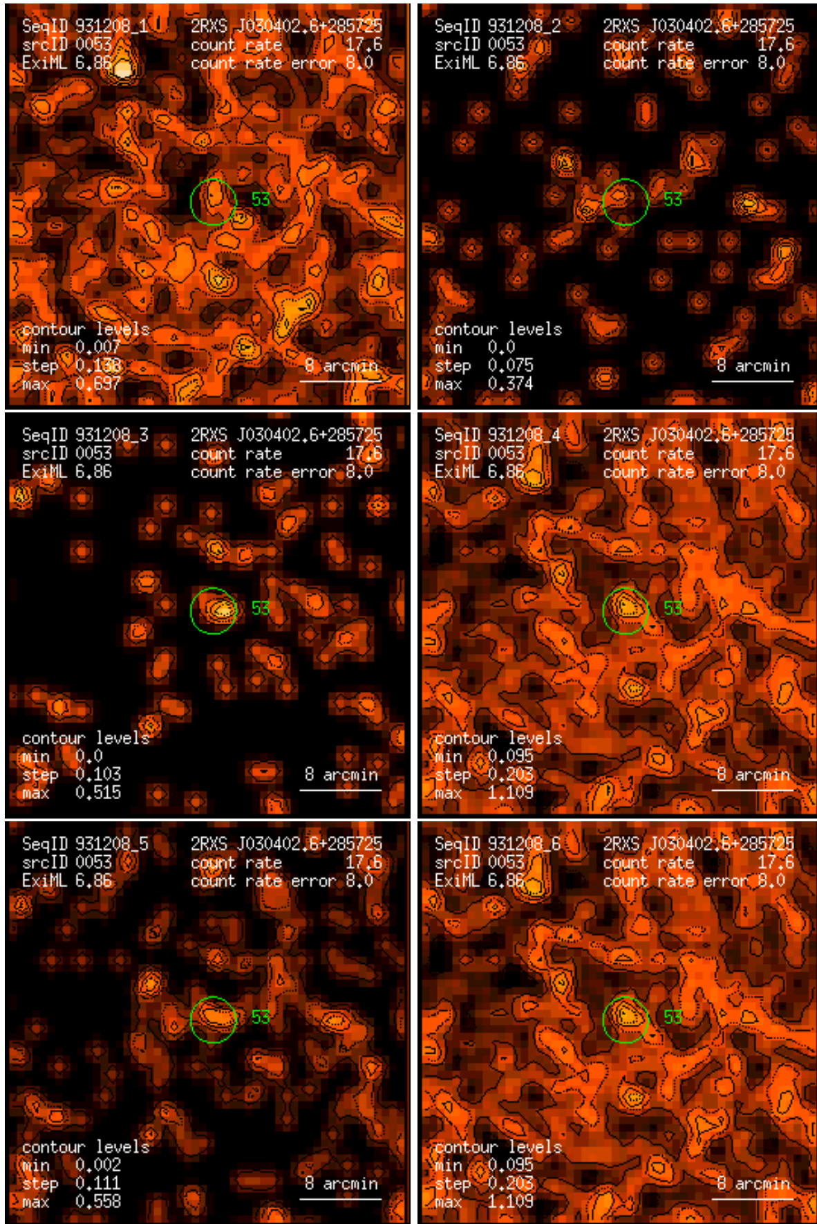
Figure 53: RASS 931208: detection 0053: band rate images, Gaussian filter: (1) PSPC channels 11 – 41, (2) 52 – 90, (3) 91 – 201, (4) 11 – 235, (5) 52 – 201, (6) 11 – 201. Broad band rates in counts/ks. Band rate contour levels in counts/ks/arcmin 2 .
