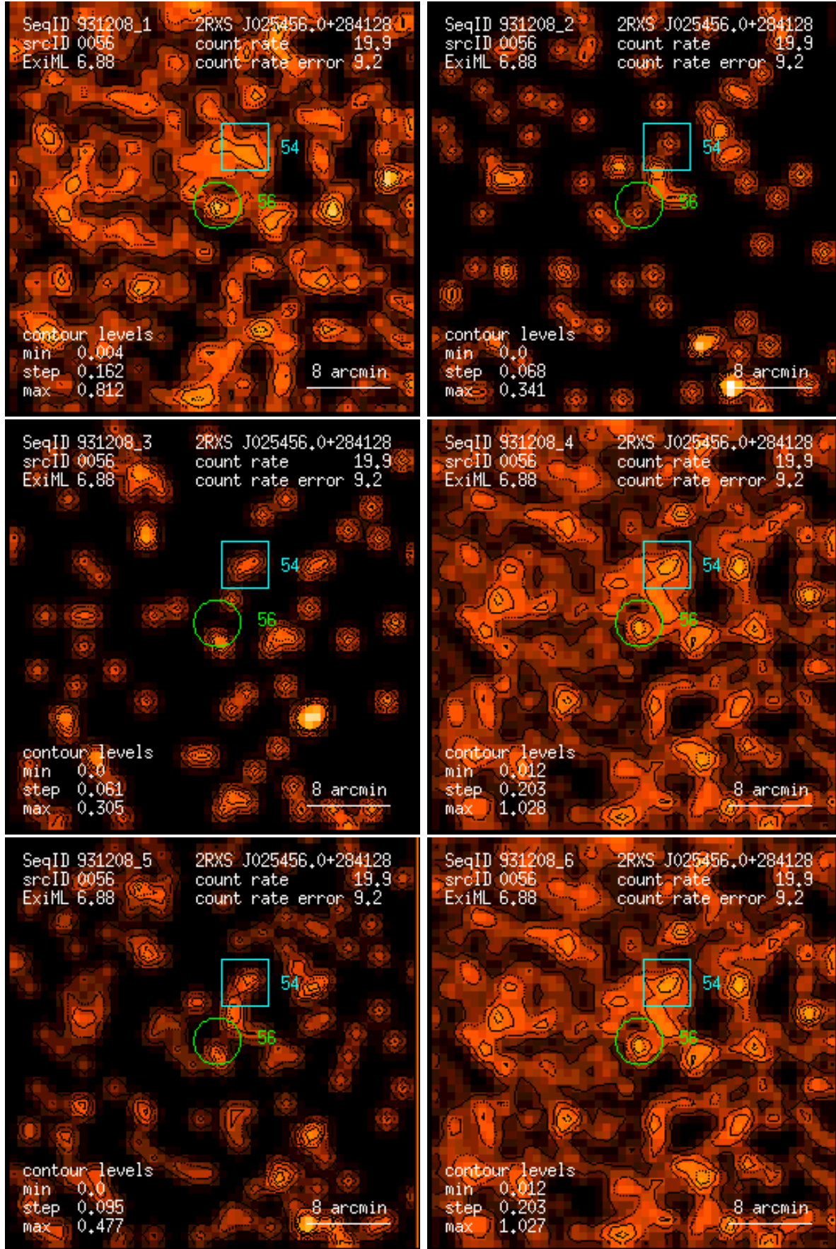
Figure 56: RASS 931208: detection 0056: band rate images, Gaussian filter: (1) PSPC channels 11 – 41, (2) 52 – 90, (3) 91 – 201, (4) 11 – 235, (5) 52 – 201, (6) 11 – 201. Broad band rates in counts/ks. Band rate contour levels in counts/ks/arcmin 2 .
