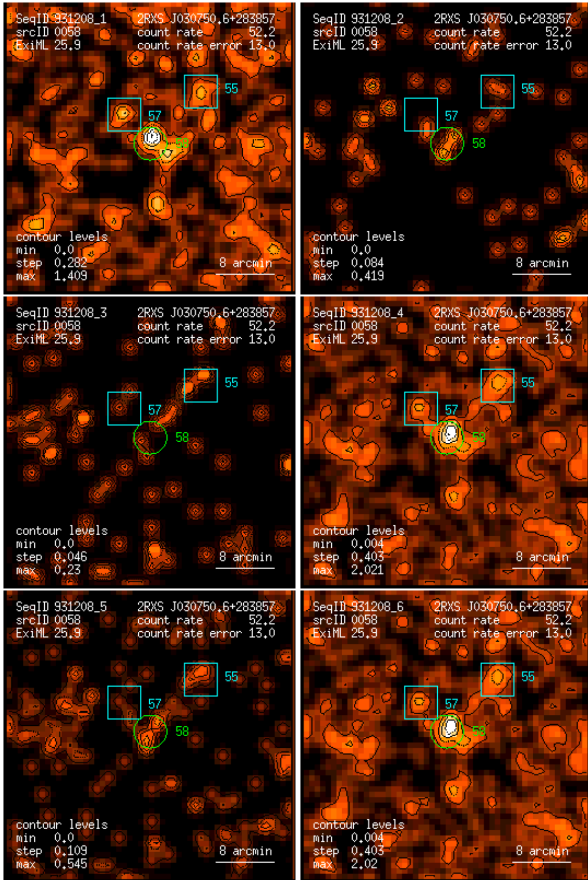
Figure 58: RASS 931208: detection 0058: band rate images, Gaussian filter: (1) PSPC channels 11 – 41, (2) 52 – 90, (3) 91 – 201, (4) 11 – 235, (5) 52 – 201, (6) 11 – 201. Broad band rates in counts/ks. Band rate contour levels in counts/ks/arcmin 2 .
