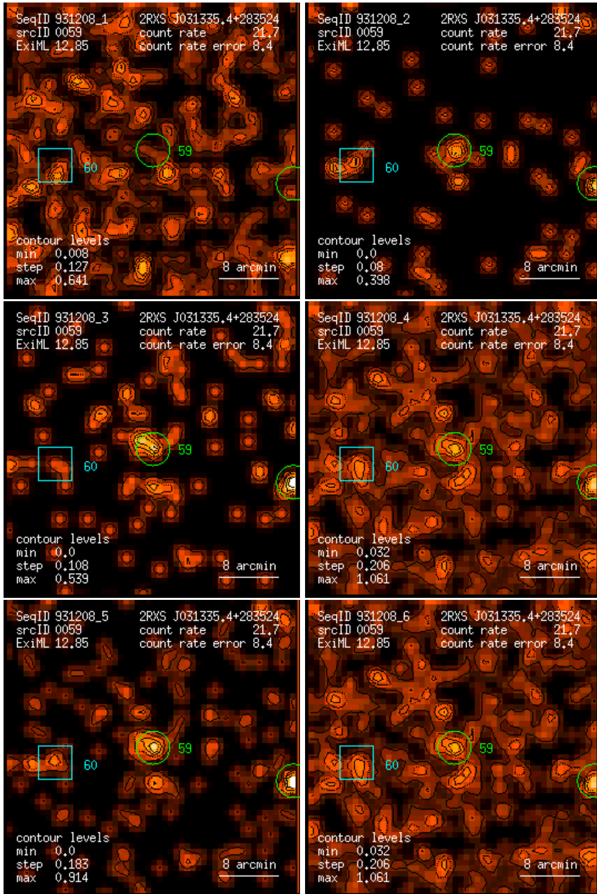
Figure 59: RASS 931208: detection 0059: band rate images, Gaussian filter: (1) PSPC channels 11 – 41, (2) 52 – 90, (3) 91 – 201, (4) 11 – 235, (5) 52 – 201, (6) 11 – 201. Broad band rates in counts/ks. Band rate contour levels in counts/ks/arcmin 2 .
