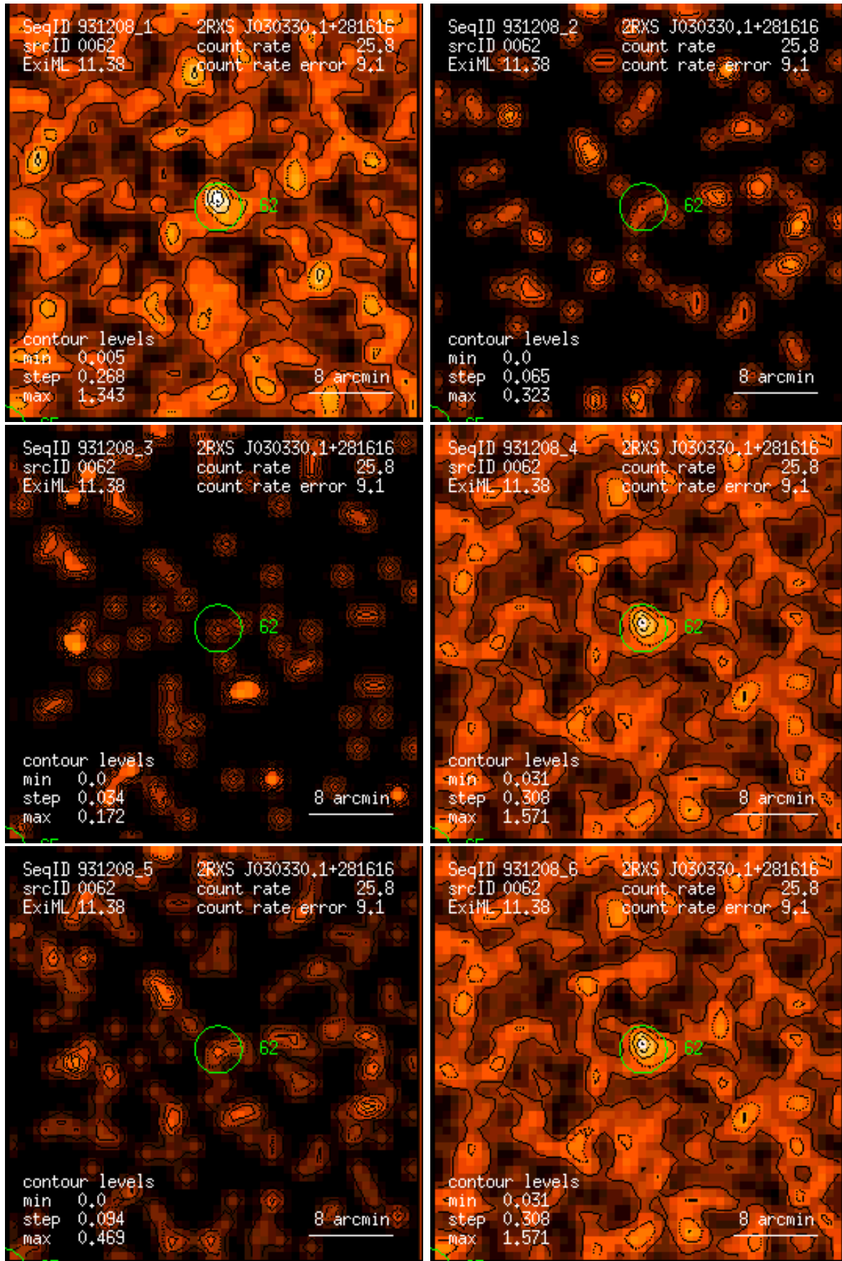
Figure 62: RASS 931208: detection 0062: band rate images, Gaussian filter: (1) PSPC channels 11 – 41, (2) 52 – 90, (3) 91 – 201, (4) 11 – 235, (5) 52 – 201, (6) 11 – 201. Broad band rates in counts/ks. Band rate contour levels in counts/ks/arcmin 2 .
