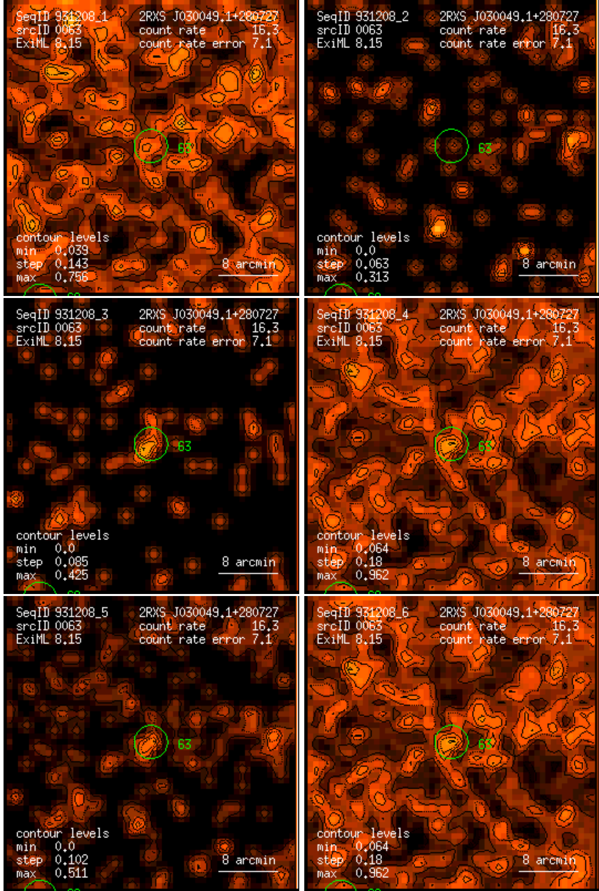
Figure 63: RASS 931208: detection 0063: band rate images, Gaussian filter: (1) PSPC channels 11 – 41, (2) 52 – 90, (3) 91 – 201, (4) 11 – 235, (5) 52 – 201, (6) 11 – 201. Broad band rates in counts/ks. Band rate contour levels in counts/ks/arcmin 2 .
