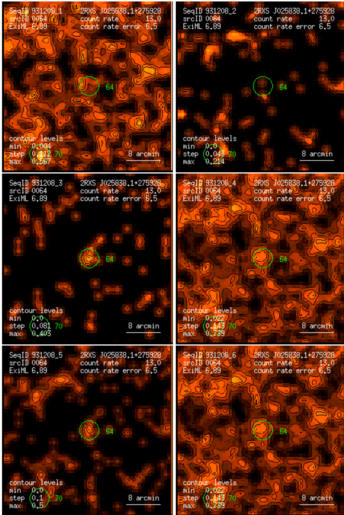
Figure 64: RASS 931208: detection 0064: band rate images, Gaussian filter: (1) PSPC channels 11 – 41, (2) 52 – 90, (3) 91 – 201, (4) 11 – 235, (5) 52 – 201, (6) 11 – 201. Broad band rates in counts/ks. Band rate contour levels in counts/ks/arcmin 2 .
