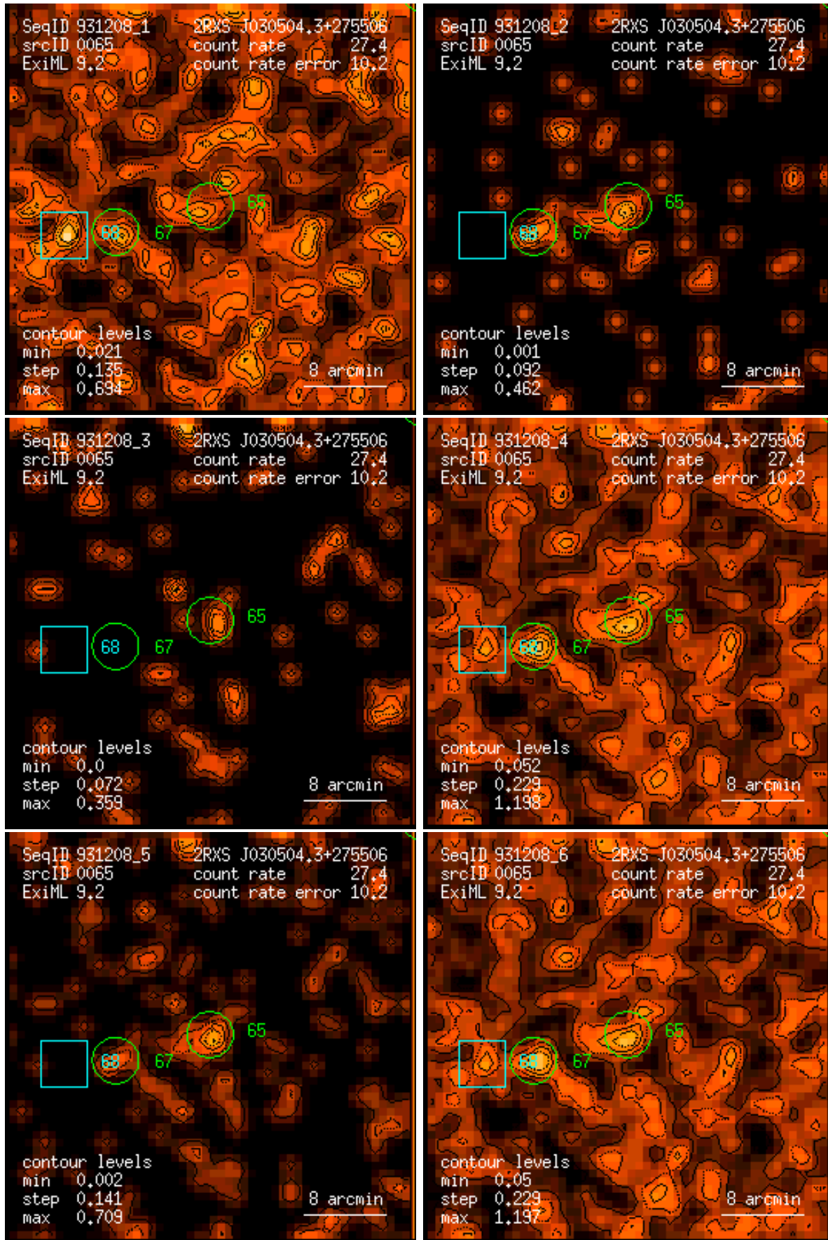
Figure 65: RASS 931208: detection 0065: band rate images, Gaussian filter: (1) PSPC channels 11 – 41, (2) 52 – 90, (3) 91 – 201, (4) 11 – 235, (5) 52 – 201, (6) 11 – 201. Broad band rates in counts/ks. Band rate contour levels in counts/ks/arcmin 2 .
