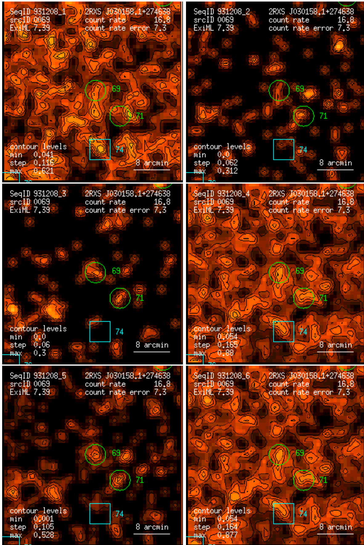
Figure 69: RASS 931208: detection 0069: band rate images, Gaussian filter: (1) PSPC channels 11 – 41, (2) 52 – 90, (3) 91 – 201, (4) 11 – 235, (5) 52 – 201, (6) 11 – 201. Broad band rates in counts/ks. Band rate contour levels in counts/ks/arcmin 2 .
