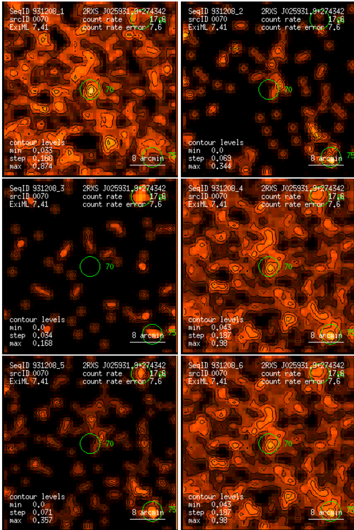
Figure 70: RASS 931208: detection 0070: band rate images, Gaussian filter: (1) PSPC channels 11 – 41, (2) 52 – 90, (3) 91 – 201, (4) 11 – 235, (5) 52 – 201, (6) 11 – 201. Broad band rates in counts/ks. Band rate contour levels in counts/ks/arcmin 2 .
