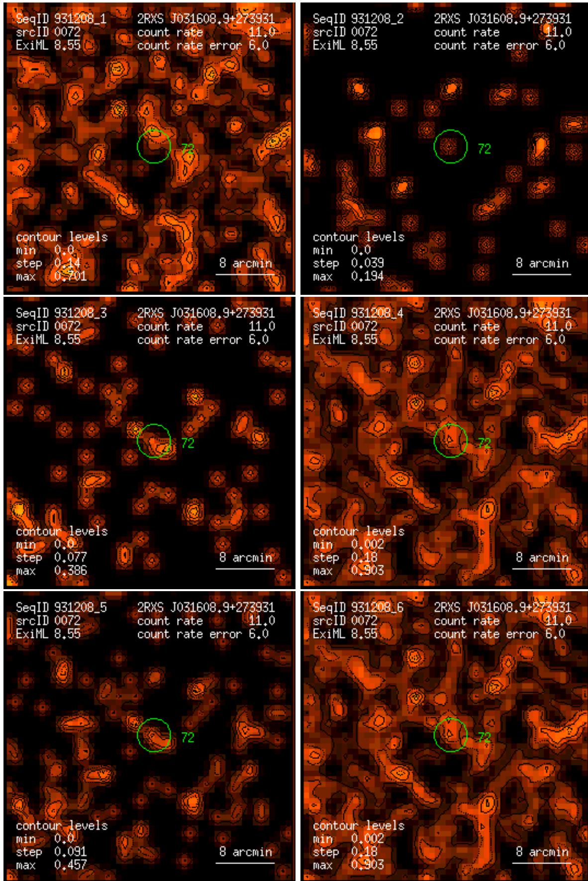
Figure 72: RASS 931208: detection 0072: band rate images, Gaussian filter: (1) PSPC channels 11 – 41, (2) 52 – 90, (3) 91 – 201, (4) 11 – 235, (5) 52 – 201, (6) 11 – 201. Broad band rates in counts/ks. Band rate contour levels in counts/ks/arcmin 2 .
