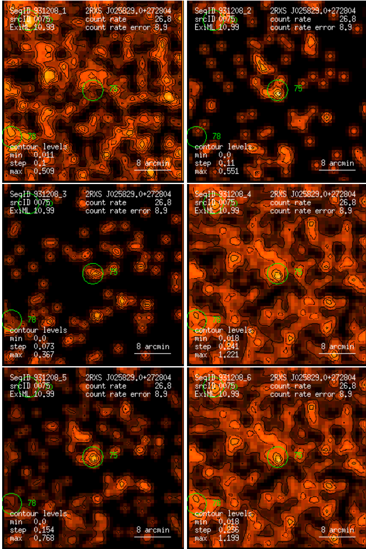
Figure 75: RASS 931208: detection 0075: band rate images, Gaussian filter: (1) PSPC channels 11 – 41, (2) 52 – 90, (3) 91 – 201, (4) 11 – 235, (5) 52 – 201, (6) 11 – 201. Broad band rates in counts/ks. Band rate contour levels in counts/ks/arcmin 2 .
