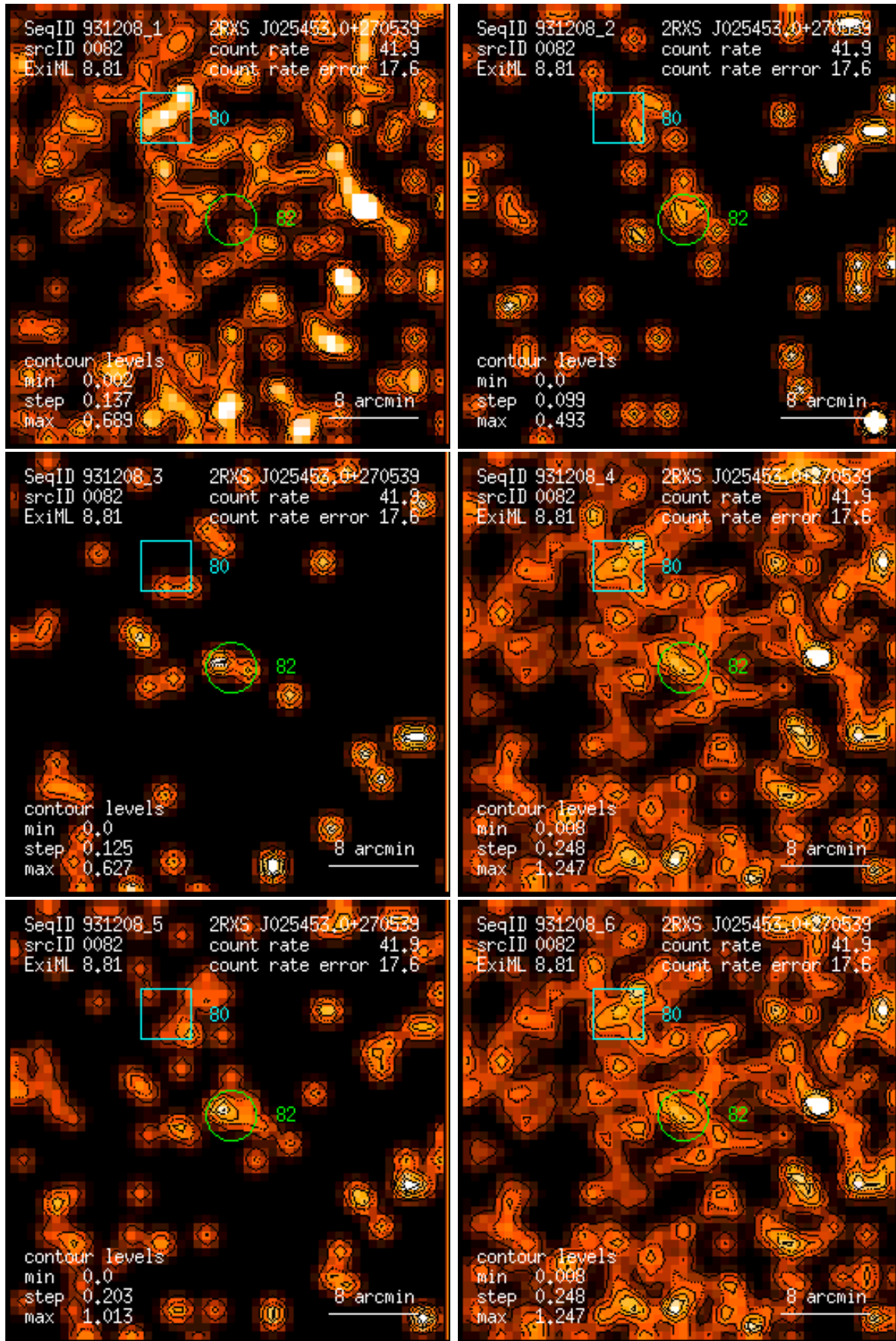
Figure 82: RASS 931208: detection 0082: band rate images, Gaussian filter: (1) PSPC channels 11 – 41, (2) 52 – 90, (3) 91 – 201, (4) 11 – 235, (5) 52 – 201, (6) 11 – 201. Broad band rates in counts/ks. Band rate contour levels in counts/ks/arcmin 2 .
