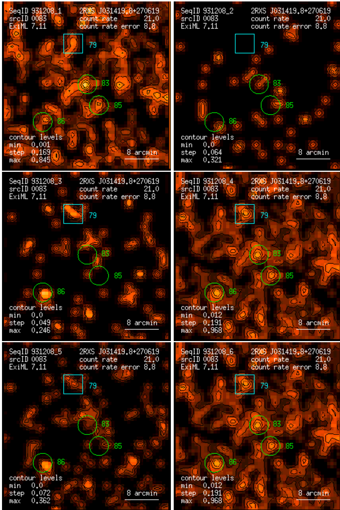
Figure 83: RASS 931208: detection 0083: band rate images, Gaussian filter: (1) PSPC channels 11 – 41, (2) 52 – 90, (3) 91 – 201, (4) 11 – 235, (5) 52 – 201, (6) 11 – 201. Broad band rates in counts/ks. Band rate contour levels in counts/ks/arcmin 2 .
