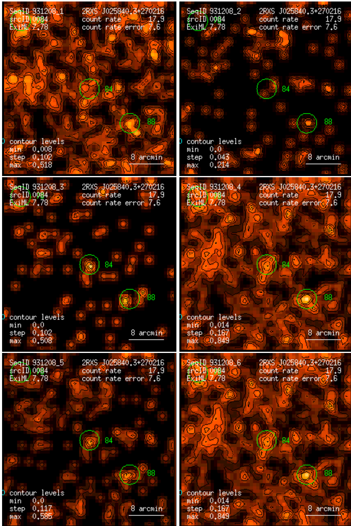
Figure 84: RASS 931208: detection 0084: band rate images, Gaussian filter: (1) PSPC channels 11 – 41, (2) 52 – 90, (3) 91 – 201, (4) 11 – 235, (5) 52 – 201, (6) 11 – 201. Broad band rates in counts/ks. Band rate contour levels in counts/ks/arcmin 2 .
