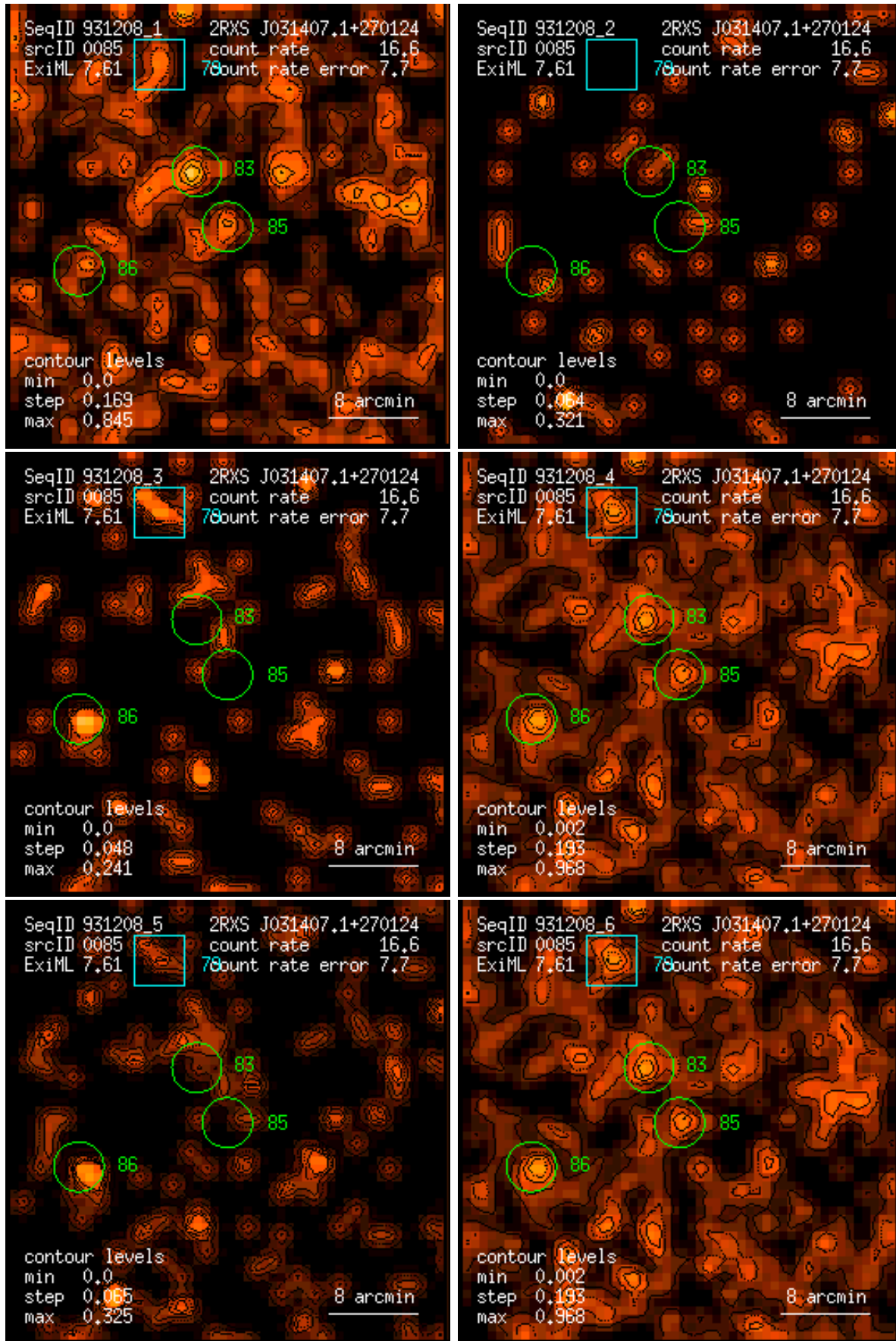
Figure 85: RASS 931208: detection 0085: band rate images, Gaussian filter: (1) PSPC channels 11 – 41, (2) 52 – 90, (3) 91 – 201, (4) 11 – 235, (5) 52 – 201, (6) 11 – 201. Broad band rates in counts/ks. Band rate contour levels in counts/ks/arcmin 2 .
