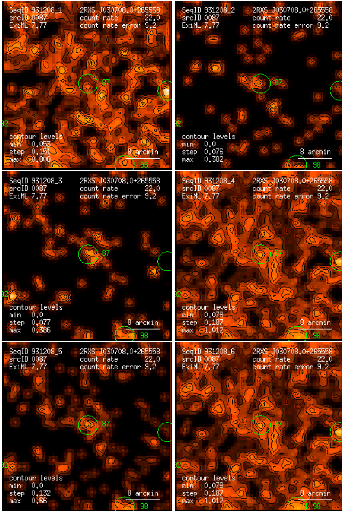
Figure 87: RASS 931208: detection 0087: band rate images, Gaussian filter: (1) PSPC channels 11 – 41, (2) 52 – 90, (3) 91 – 201, (4) 11 – 235, (5) 52 – 201, (6) 11 – 201. Broad band rates in counts/ks. Band rate contour levels in counts/ks/arcmin 2 .
