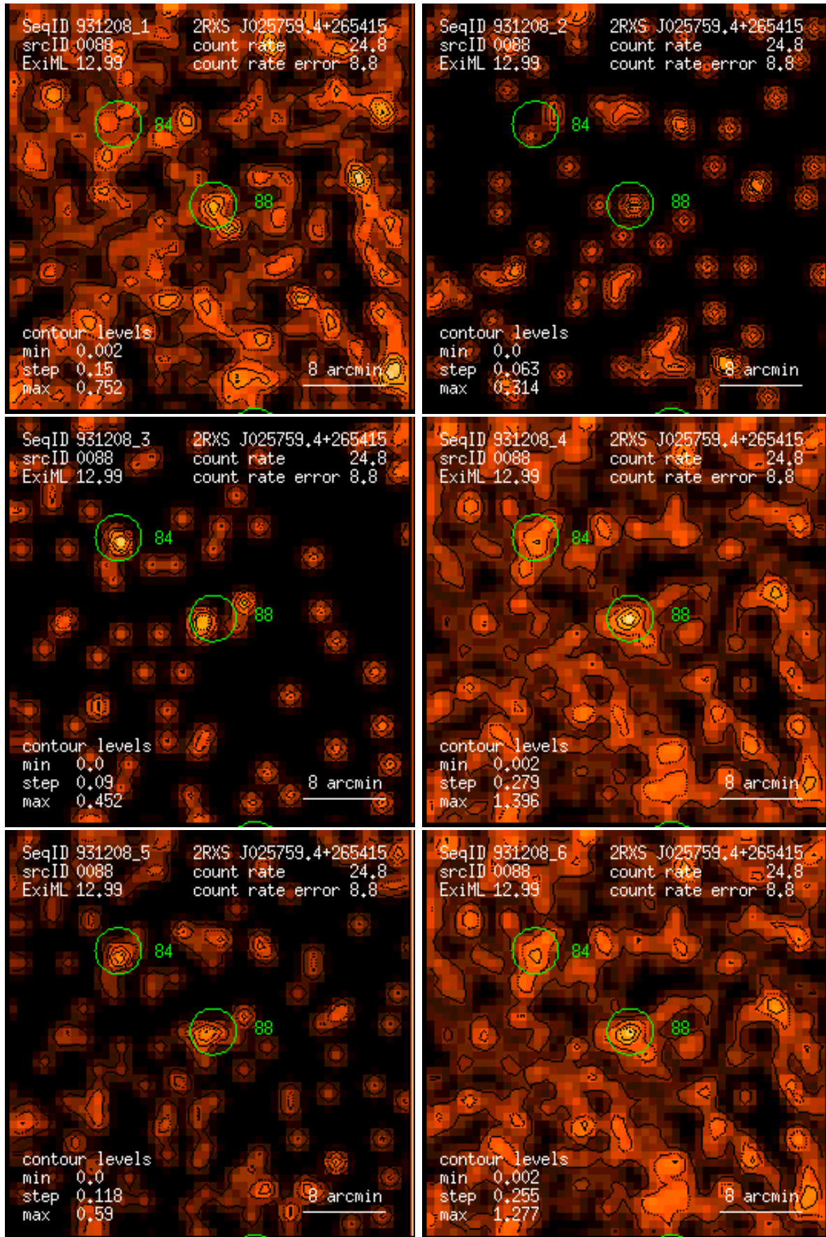
Figure 88: RASS 931208: detection 0088: band rate images, Gaussian filter: (1) PSPC channels 11 – 41, (2) 52 – 90, (3) 91 – 201, (4) 11 – 235, (5) 52 – 201, (6) 11 – 201. Broad band rates in counts/ks. Band rate contour levels in counts/ks/arcmin 2 .
