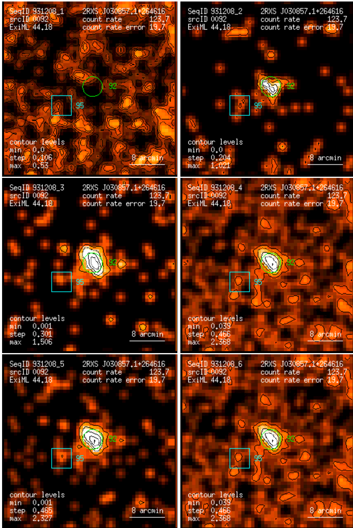
Figure 92: RASS 931208: detection 0092: band rate images, Gaussian filter: (1) PSPC channels 11 – 41, (2) 52 – 90, (3) 91 – 201, (4) 11 – 235, (5) 52 – 201, (6) 11 – 201. Broad band rates in counts/ks. Band rate contour levels in counts/ks/arcmin 2 .
