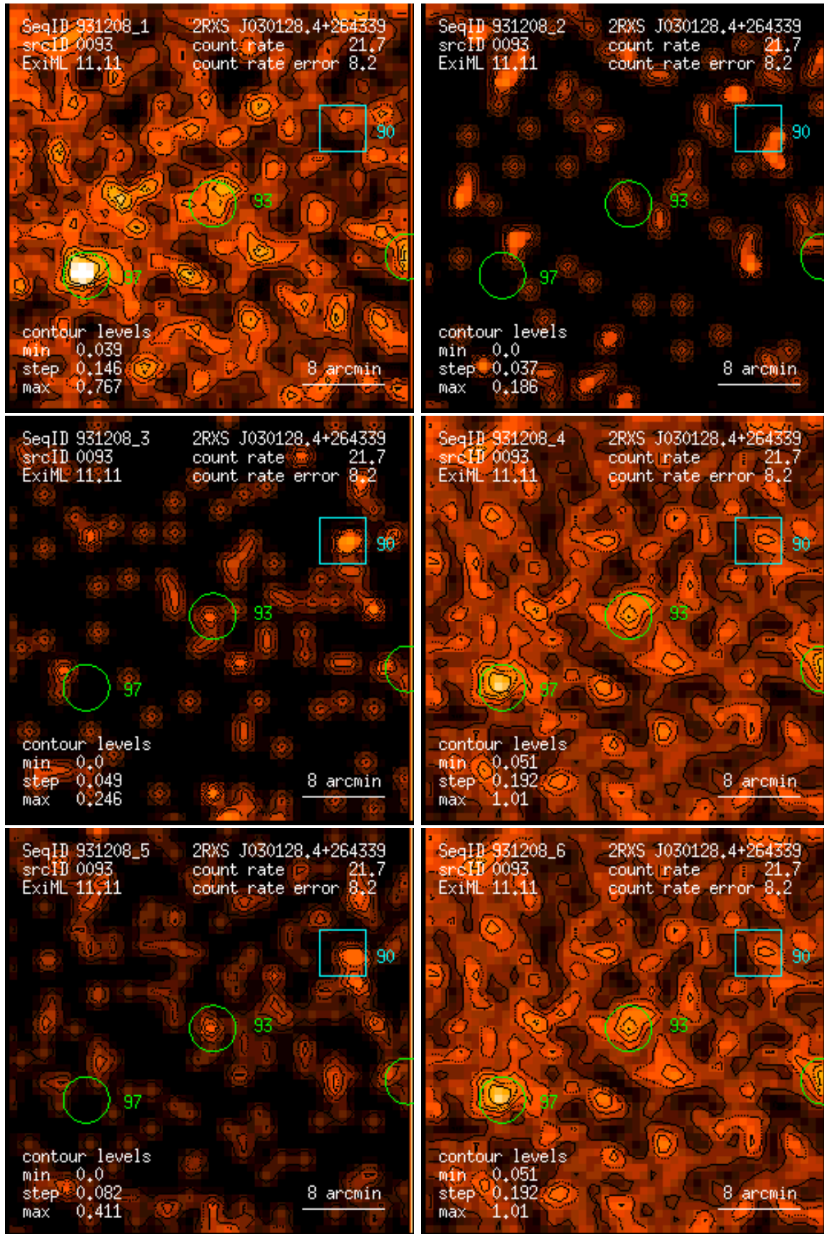
Figure 93: RASS 931208: detection 0093: band rate images, Gaussian filter: (1) PSPC channels 11 – 41, (2) 52 – 90, (3) 91 – 201, (4) 11 – 235, (5) 52 – 201, (6) 11 – 201. Broad band rates in counts/ks. Band rate contour levels in counts/ks/arcmin 2 .
