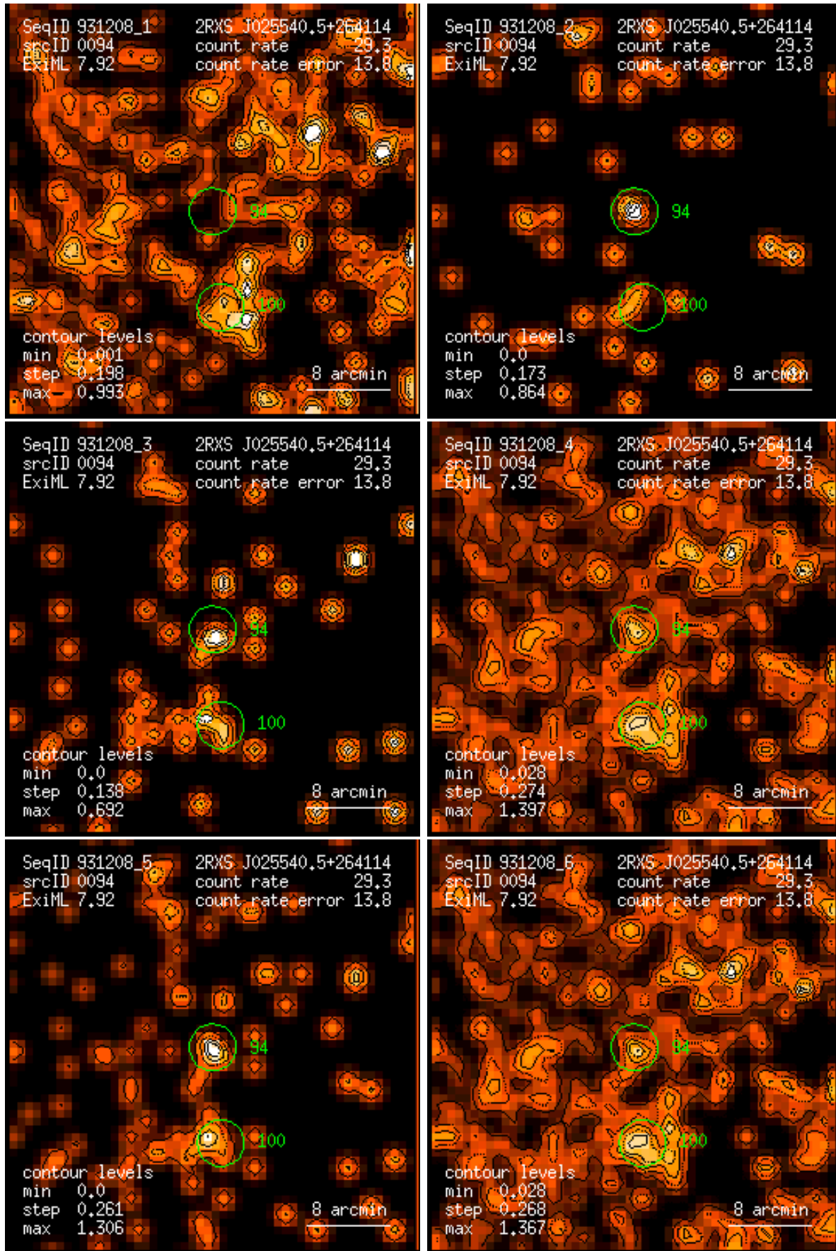
Figure 94: RASS 931208: detection 0094: band rate images, Gaussian filter: (1) PSPC channels 11 – 41, (2) 52 – 90, (3) 91 – 201, (4) 11 – 235, (5) 52 – 201, (6) 11 – 201. Broad band rates in counts/ks. Band rate contour levels in counts/ks/arcmin 2 .
