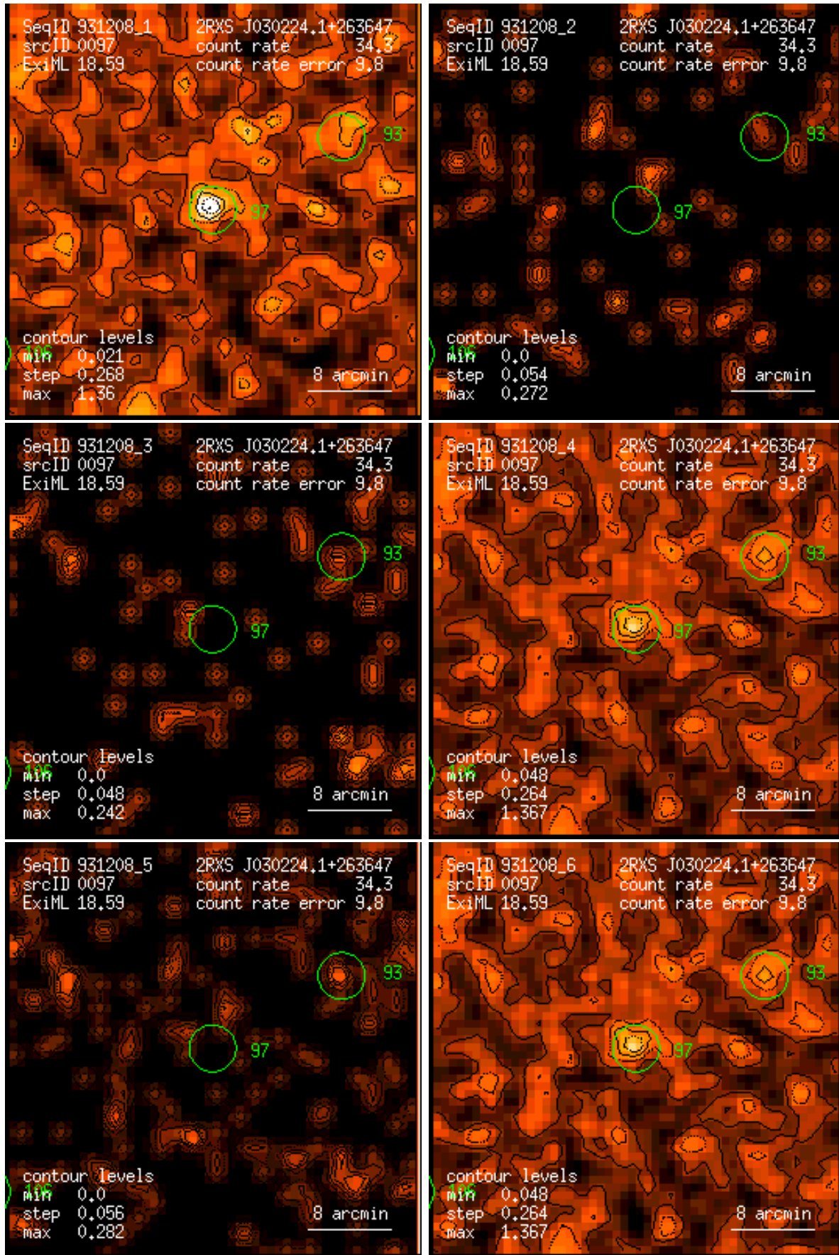
Figure 97: RASS 931208: detection 0097: band rate images, Gaussian filter: (1) PSPC channels 11 – 41, (2) 52 – 90, (3) 91 – 201, (4) 11 – 235, (5) 52 – 201, (6) 11 – 201. Broad band rates in counts/ks. Band rate contour levels in counts/ks/arcmin 2 .
