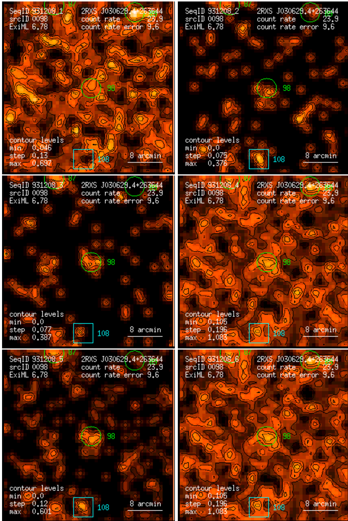
Figure 98: RASS 931208: detection 0098: band rate images, Gaussian filter: (1) PSPC channels 11 – 41, (2) 52 – 90, (3) 91 – 201, (4) 11 – 235, (5) 52 – 201, (6) 11 – 201. Broad band rates in counts/ks. Band rate contour levels in counts/ks/arcmin 2 .
