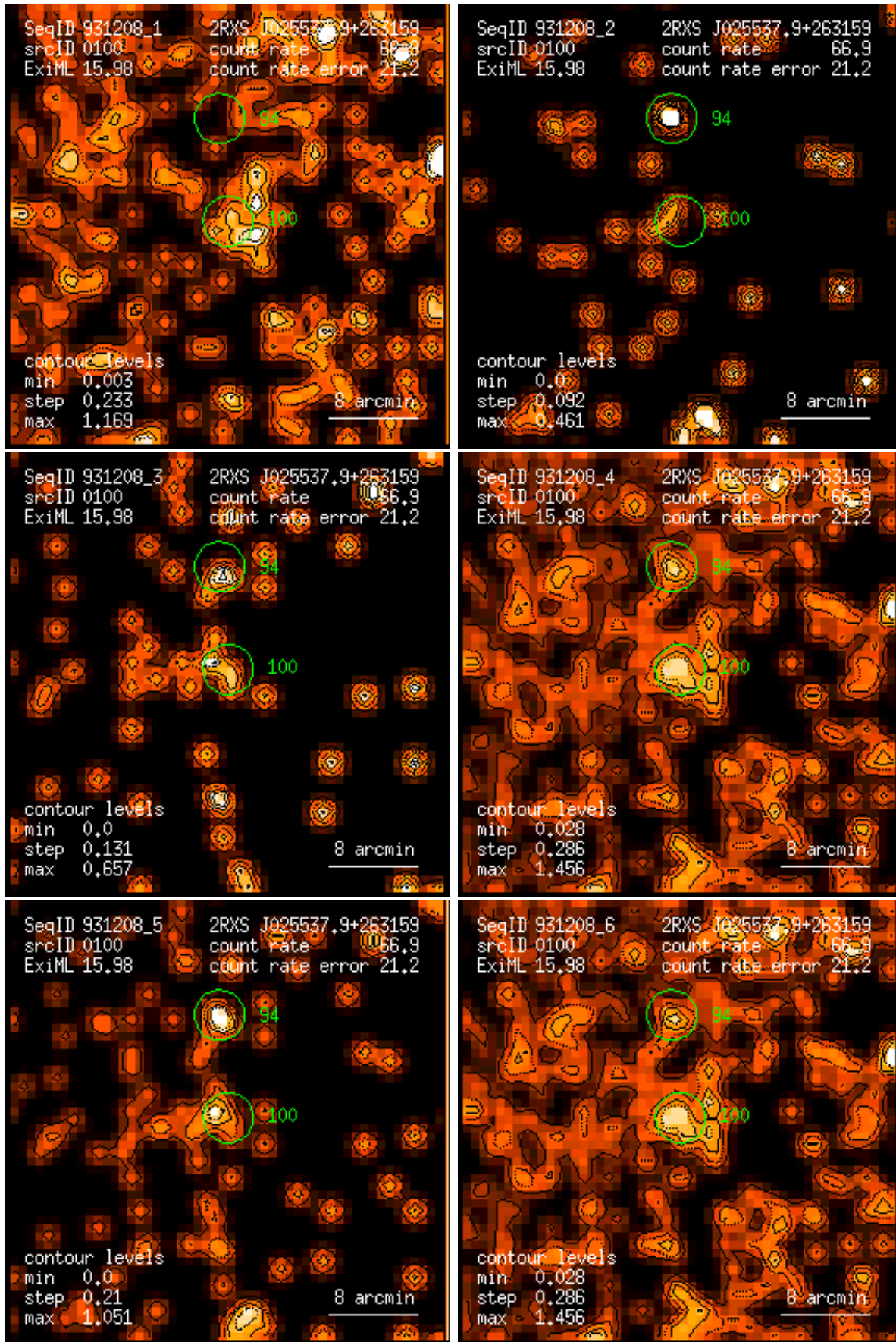
Figure 100: RASS 931208: detection 0100: band rate images, Gaussian filter: (1) PSPC channels 11 – 41, (2) 52 – 90, (3) 91 – 201, (4) 11 – 235, (5) 52 – 201, (6) 11 – 201. Broad band rates in counts/ks. Band rate contour levels in counts/ks/arcmin 2 .
