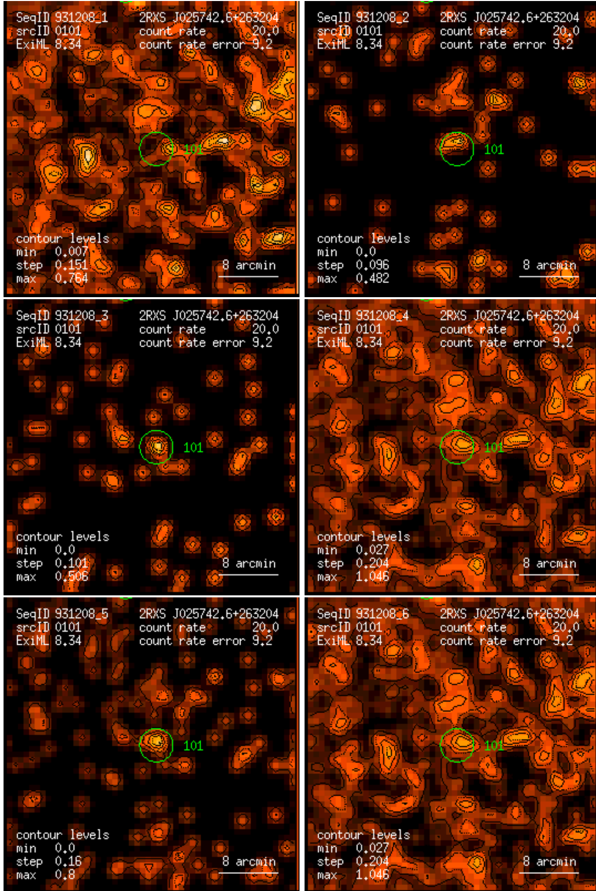
Figure 101: RASS 931208: detection 0101: band rate images, Gaussian filter: (1) PSPC channels 11 – 41, (2) 52 – 90, (3) 91 – 201, (4) 11 – 235, (5) 52 – 201, (6) 11 – 201. Broad band rates in counts/ks. Band rate contour levels in counts/ks/arcmin 2 .
