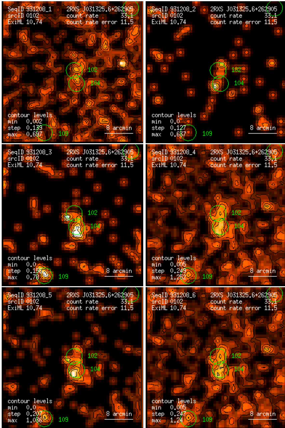
Figure 102: RASS 931208: detection 0102: band rate images, Gaussian filter: (1) PSPC channels 11 – 41, (2) 52 – 90, (3) 91 – 201, (4) 11 – 235, (5) 52 – 201, (6) 11 – 201. Broad band rates in counts/ks. Band rate contour levels in counts/ks/arcmin 2 .
