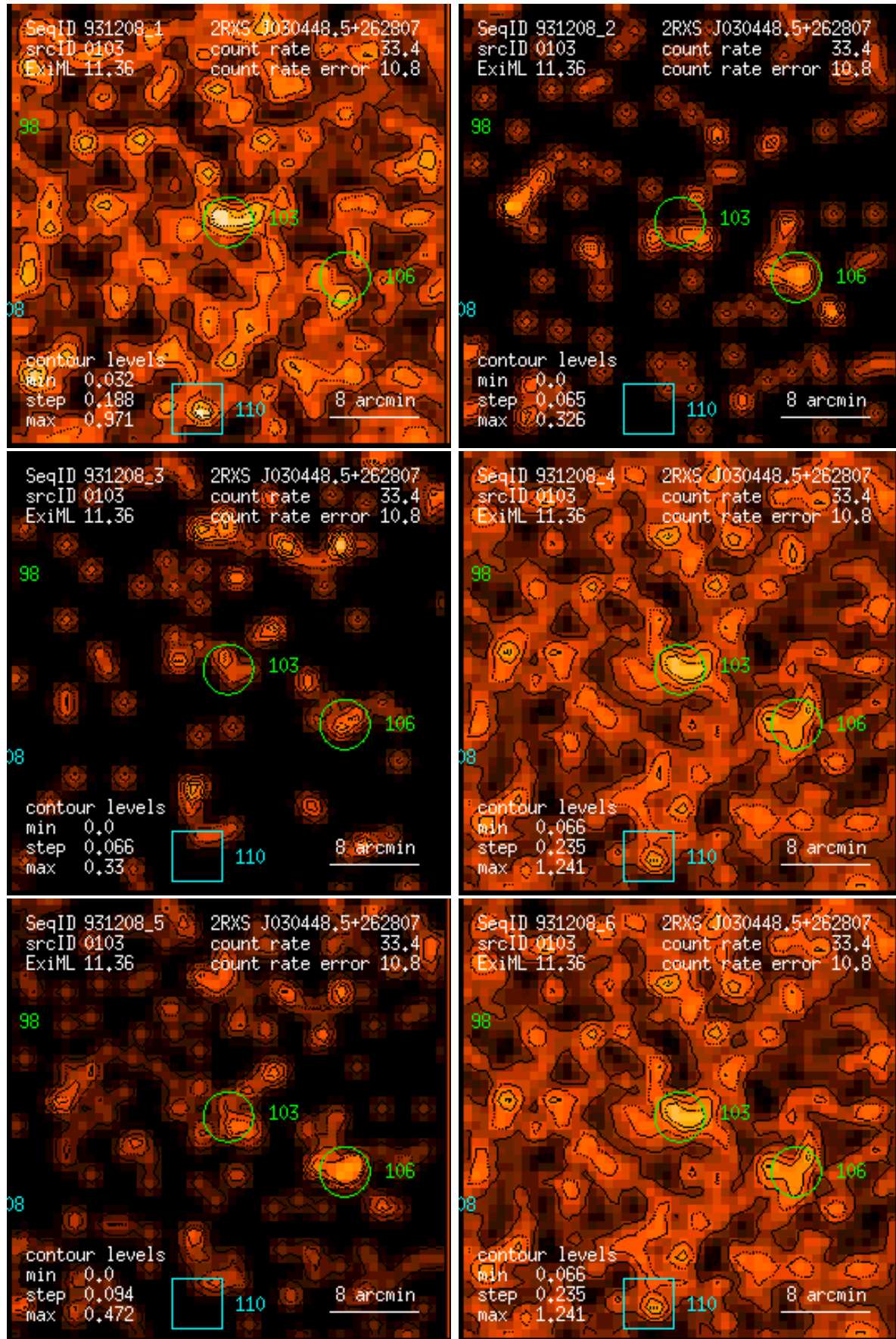
Figure 103: RASS 931208: detection 0103: band rate images, Gaussian filter: (1) PSPC channels 11 – 41, (2) 52 – 90, (3) 91 – 201, (4) 11 – 235, (5) 52 – 201, (6) 11 – 201. Broad band rates in counts/ks. Band rate contour levels in counts/ks/arcmin 2 .
