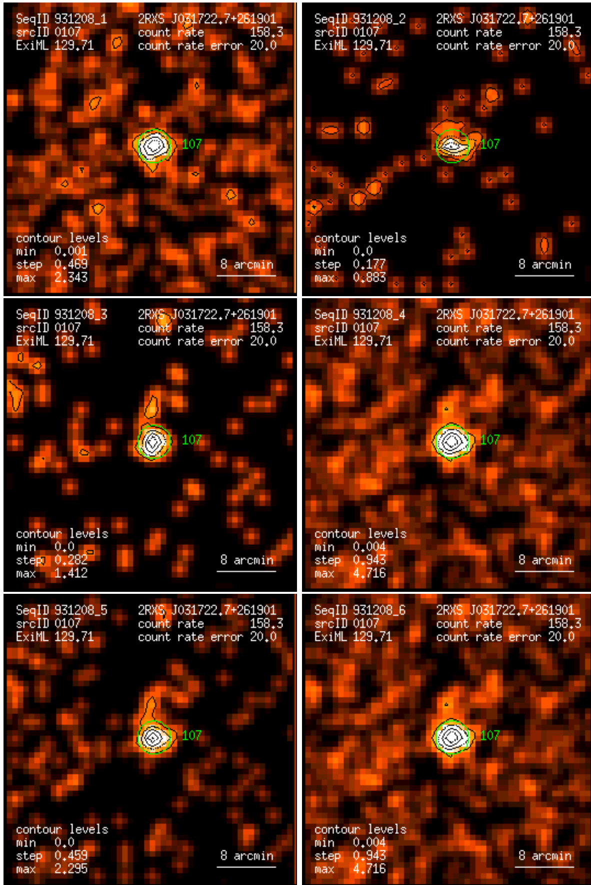
Figure 107: RASS 931208: detection 0107: band rate images, Gaussian filter: (1) PSPC channels 11 – 41, (2) 52 – 90, (3) 91 – 201, (4) 11 – 235, (5) 52 – 201, (6) 11 – 201. Broad band rates in counts/ks. Band rate contour levels in counts/ks/arcmin 2 .
