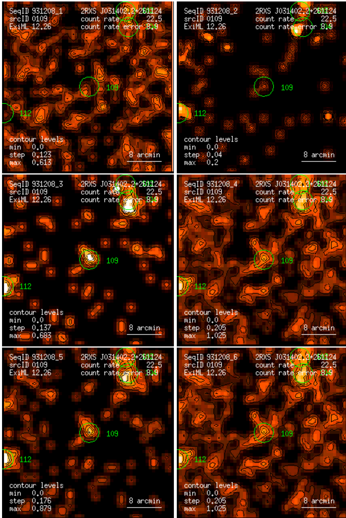
Figure 109: RASS 931208: detection 0109: band rate images, Gaussian filter: (1) PSPC channels 11 – 41, (2) 52 – 90, (3) 91 – 201, (4) 11 – 235, (5) 52 – 201, (6) 11 – 201. Broad band rates in counts/ks. Band rate contour levels in counts/ks/arcmin 2 .
