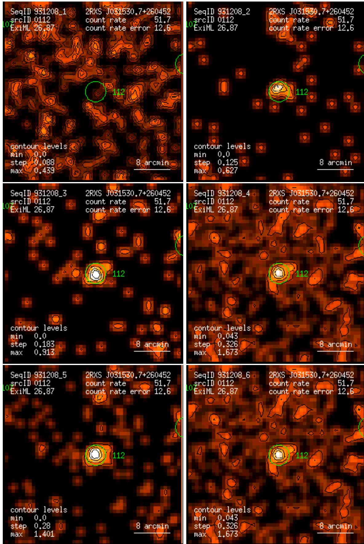
Figure 112: RASS 931208: detection 0112: band rate images, Gaussian filter: (1) PSPC channels 11 – 41, (2) 52 – 90, (3) 91 – 201, (4) 11 – 235, (5) 52 – 201, (6) 11 – 201. Broad band rates in counts/ks. Band rate contour levels in counts/ks/arcmin 2 .
