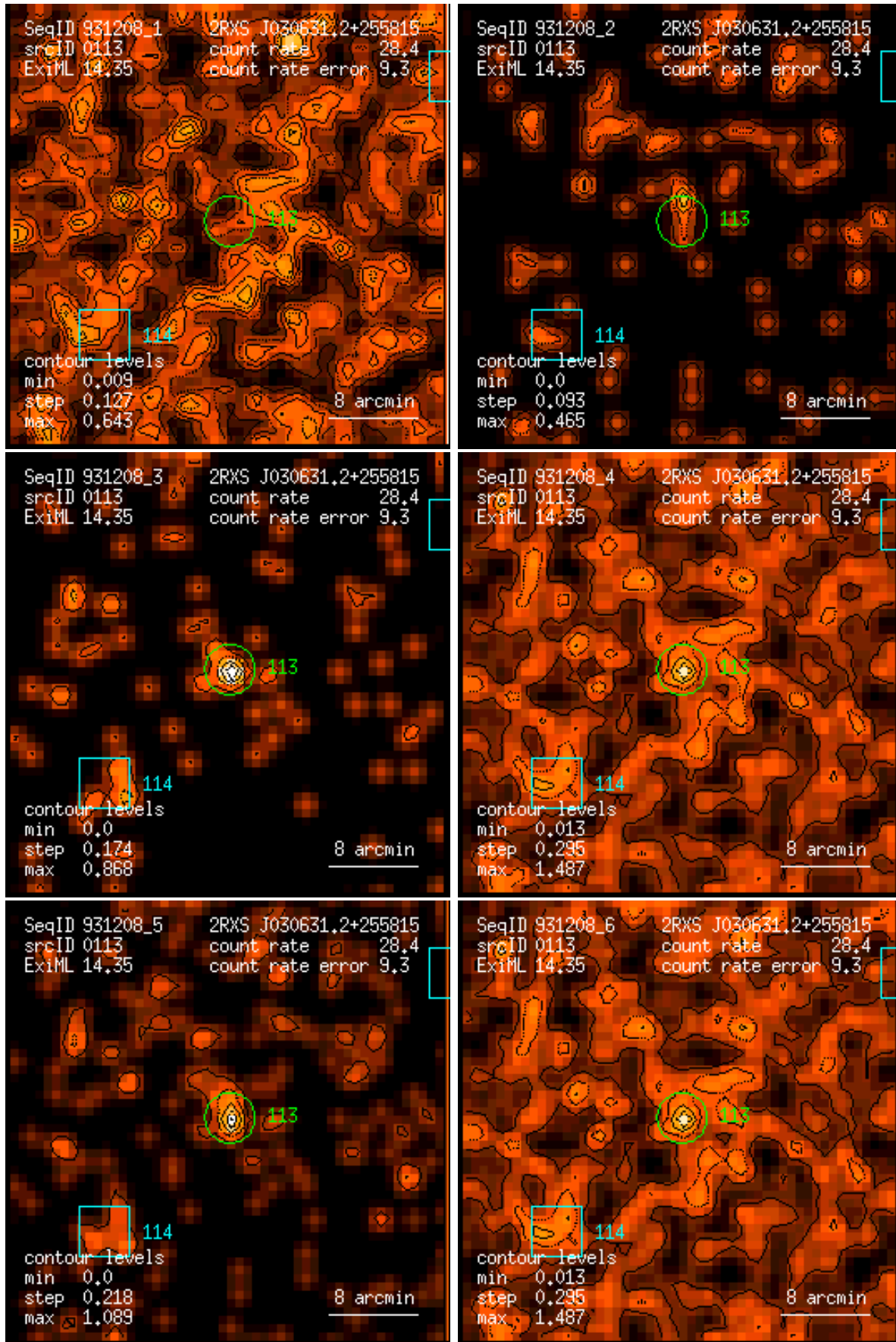
Figure 113: RASS 931208: detection 0113: band rate images, Gaussian filter: (1) PSPC channels 11 – 41, (2) 52 – 90, (3) 91 – 201, (4) 11 – 235, (5) 52 – 201, (6) 11 – 201. Broad band rates in counts/ks. Band rate contour levels in counts/ks/arcmin 2 .
