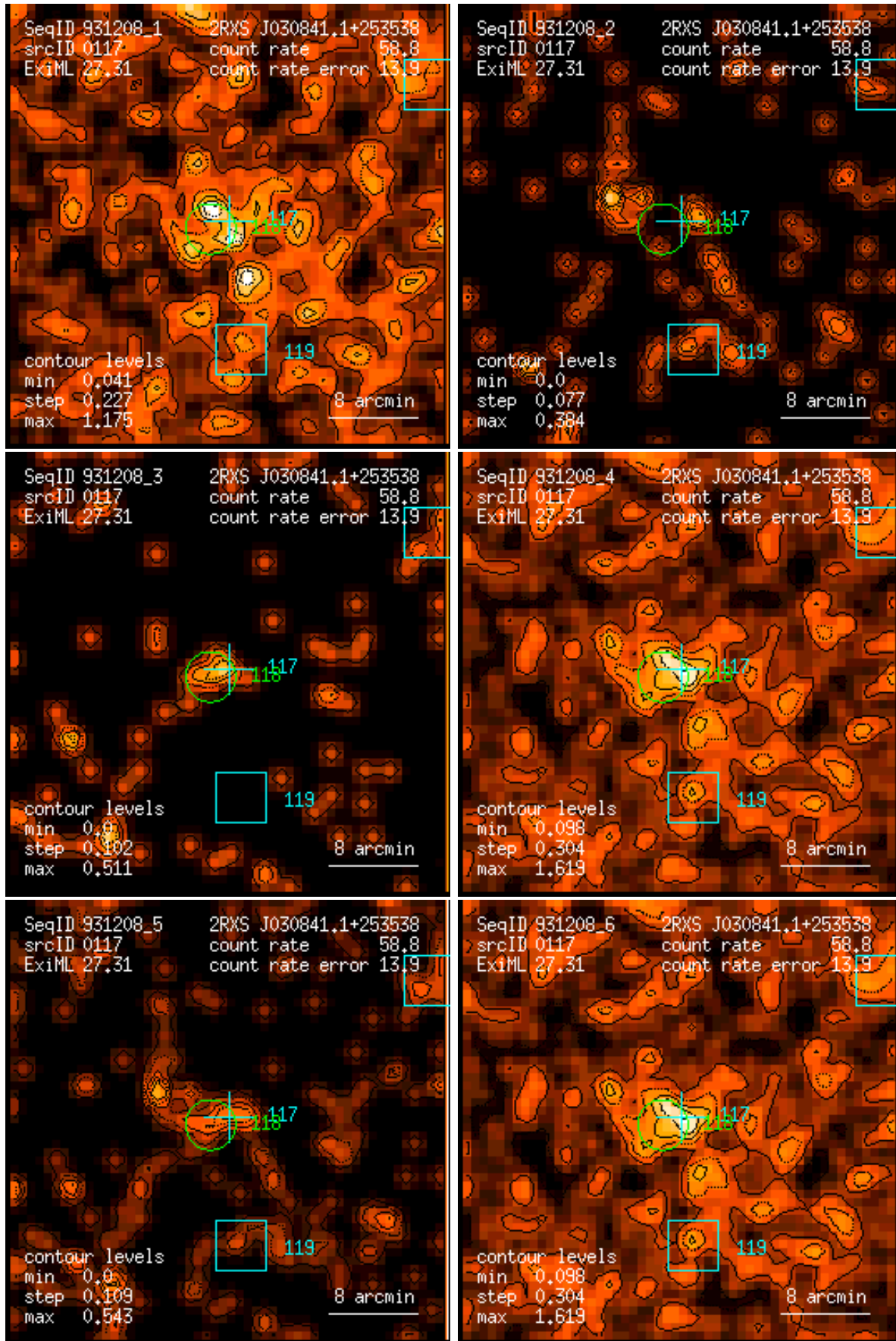
Figure 117: RASS 931208: detection 0117: band rate images, Gaussian filter: (1) PSPC channels 11 – 41, (2) 52 – 90, (3) 91 – 201, (4) 11 – 235, (5) 52 – 201, (6) 11 – 201. Broad band rates in counts/ks. Band rate contour levels in counts/ks/arcmin 2 .
