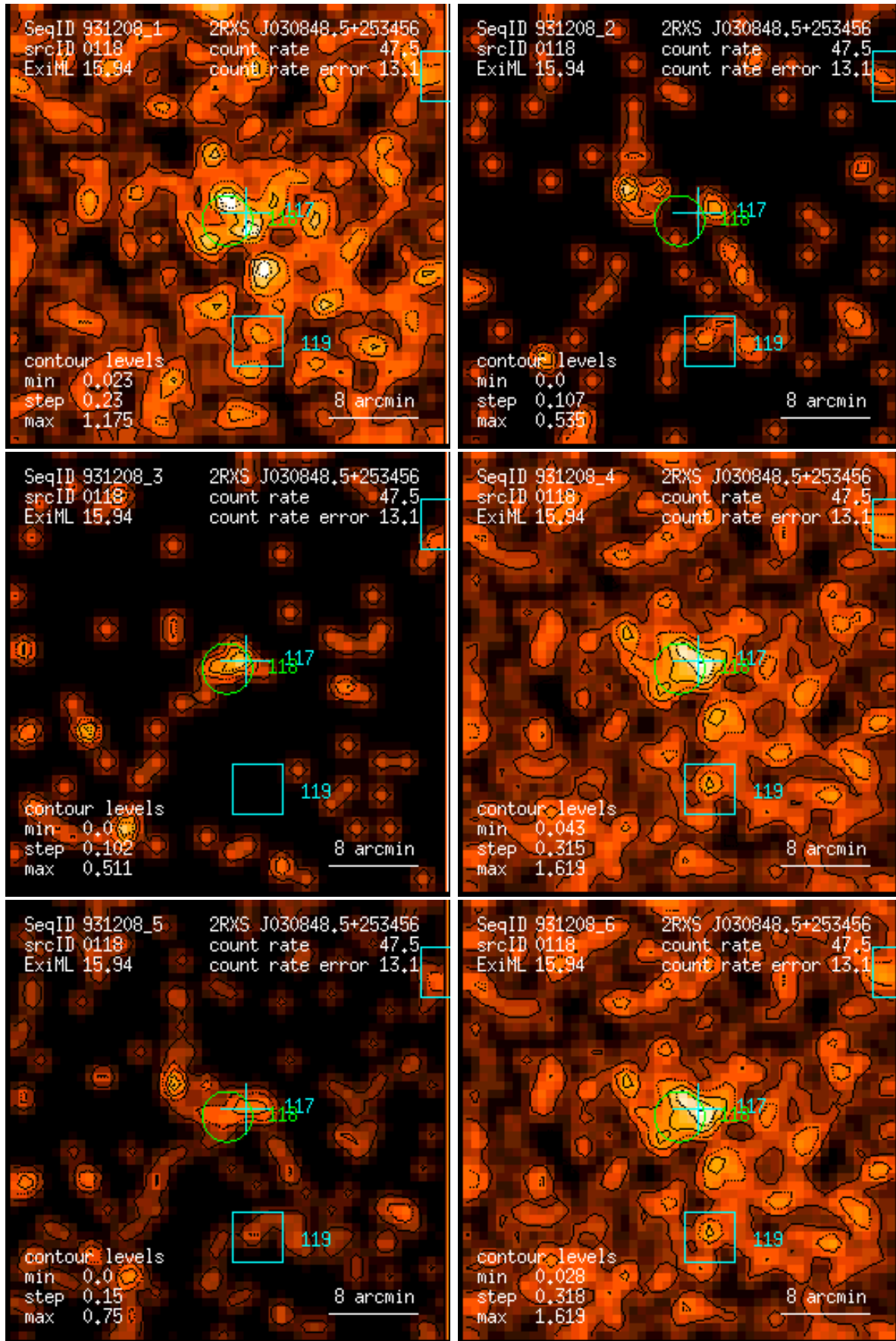
Figure 118: RASS 931208: detection 0118: band rate images, Gaussian filter: (1) PSPC channels 11 – 41, (2) 52 – 90, (3) 91 – 201, (4) 11 – 235, (5) 52 – 201, (6) 11 – 201. Broad band rates in counts/ks. Band rate contour levels in counts/ks/arcmin 2 .
