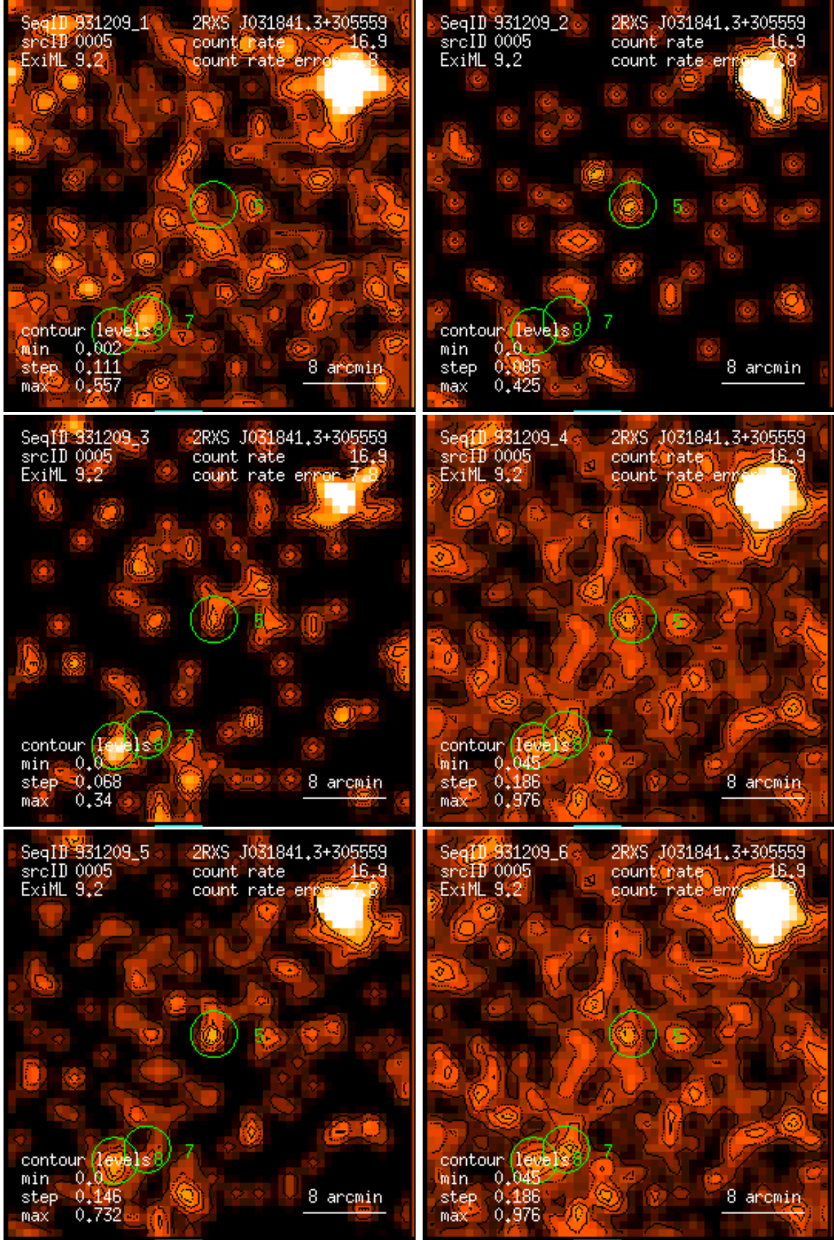
Figure 5: RASS 931209: detection 0005: band rate images, Gaussian filter: (1) PSPC channels 11 – 41, (2) 52 – 90, (3) 91 – 201, (4) 11 – 235, (5) 52 – 201, (6) 11 – 201. Broad band rates in counts/ks. Band rate contour levels in counts/ks/arcmin 2 .
