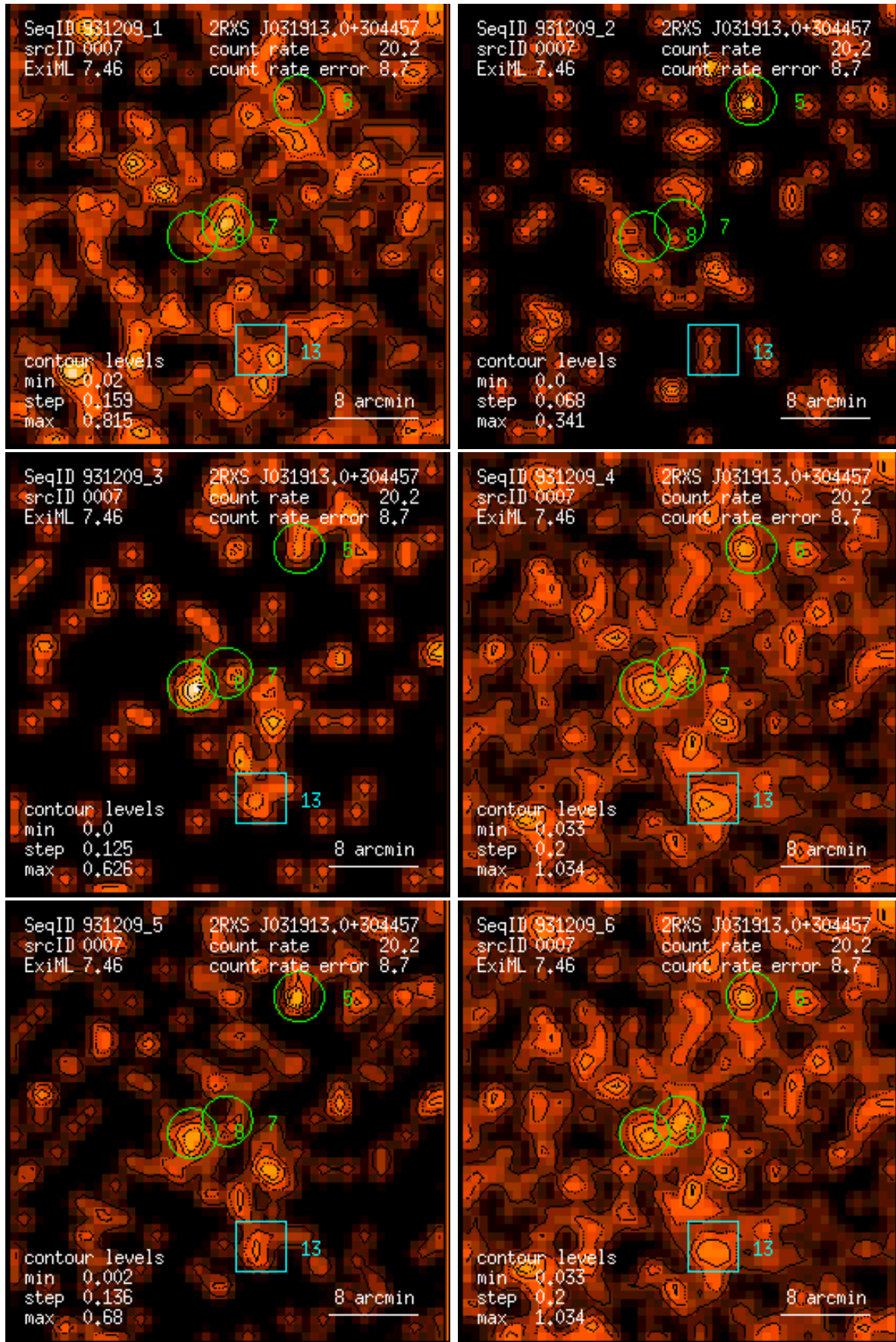
Figure 7: RASS 931209: detection 0007: band rate images, Gaussian filter: (1) PSPC channels 11 – 41, (2) 52 – 90, (3) 91 – 201, (4) 11 – 235, (5) 52 – 201, (6) 11 – 201. Broad band rates in counts/ks. Band rate contour levels in counts/ks/arcmin 2 .
