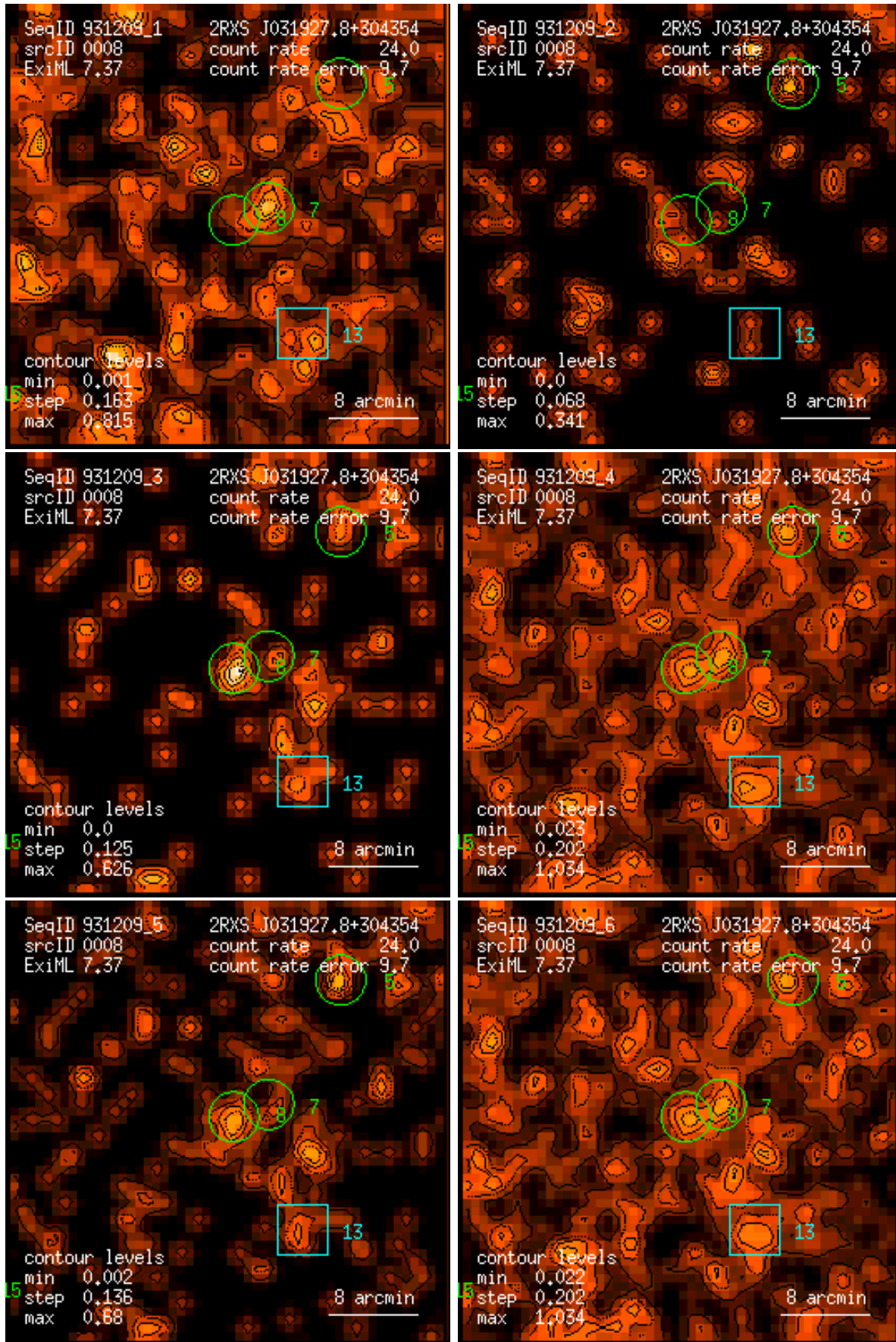
Figure 8: RASS 931209: detection 0008: band rate images, Gaussian filter: (1) PSPC channels 11 – 41, (2) 52 – 90, (3) 91 – 201, (4) 11 – 235, (5) 52 – 201, (6) 11 – 201. Broad band rates in counts/ks. Band rate contour levels in counts/ks/arcmin 2 .
