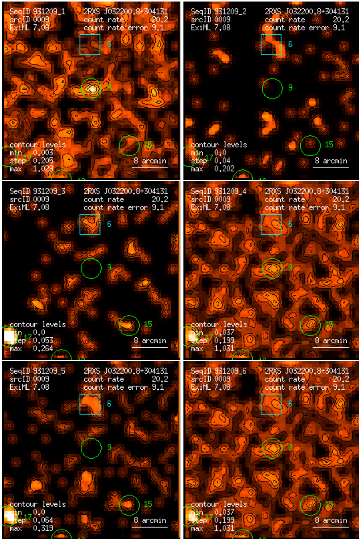
Figure 9: RASS 931209: detection 0009: band rate images, Gaussian filter: (1) PSPC channels 11 – 41, (2) 52 – 90, (3) 91 – 201, (4) 11 – 235, (5) 52 – 201, (6) 11 – 201. Broad band rates in counts/ks. Band rate contour levels in counts/ks/arcmin 2 .
