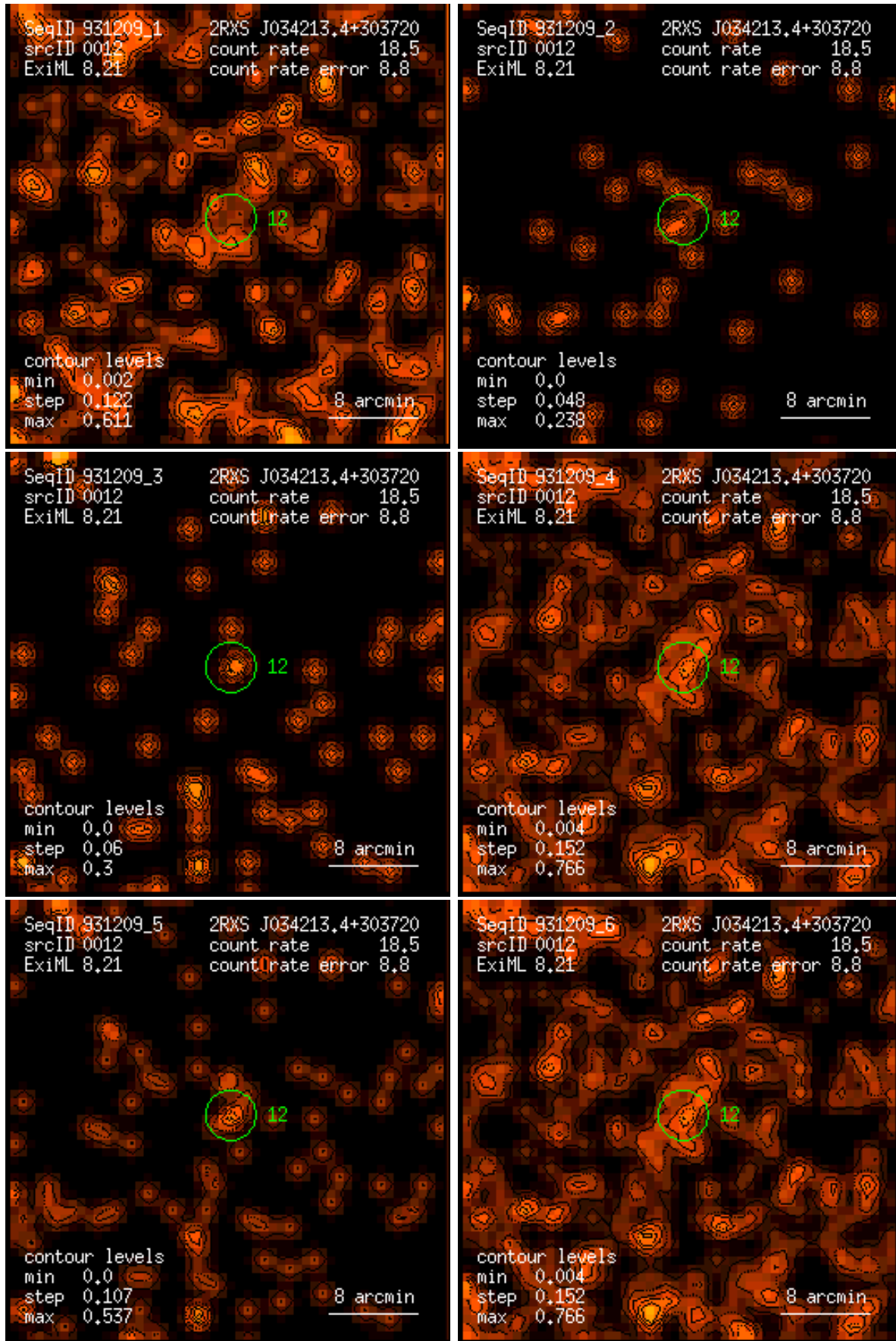
Figure 12: RASS 931209: detection 0012: band rate images, Gaussian filter: (1) PSPC channels 11 – 41, (2) 52 – 90, (3) 91 – 201, (4) 11 – 235, (5) 52 – 201, (6) 11 – 201. Broad band rates in counts/ks. Band rate contour levels in counts/ks/arcmin 2 .
