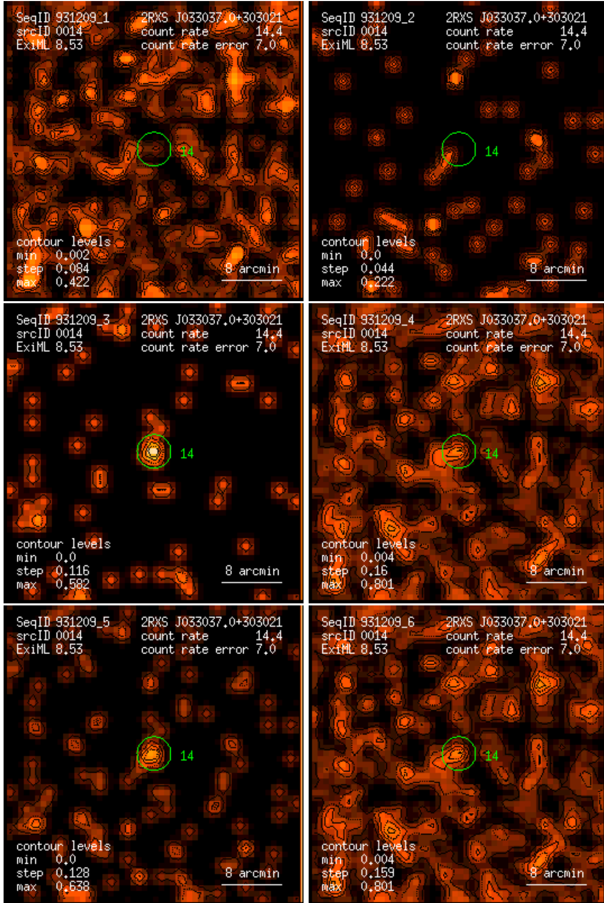
Figure 14: RASS 931209: detection 0014: band rate images, Gaussian filter: (1) PSPC channels 11 – 41, (2) 52 – 90, (3) 91 – 201, (4) 11 – 235, (5) 52 – 201, (6) 11 – 201. Broad band rates in counts/ks. Band rate contour levels in counts/ks/arcmin 2 .
