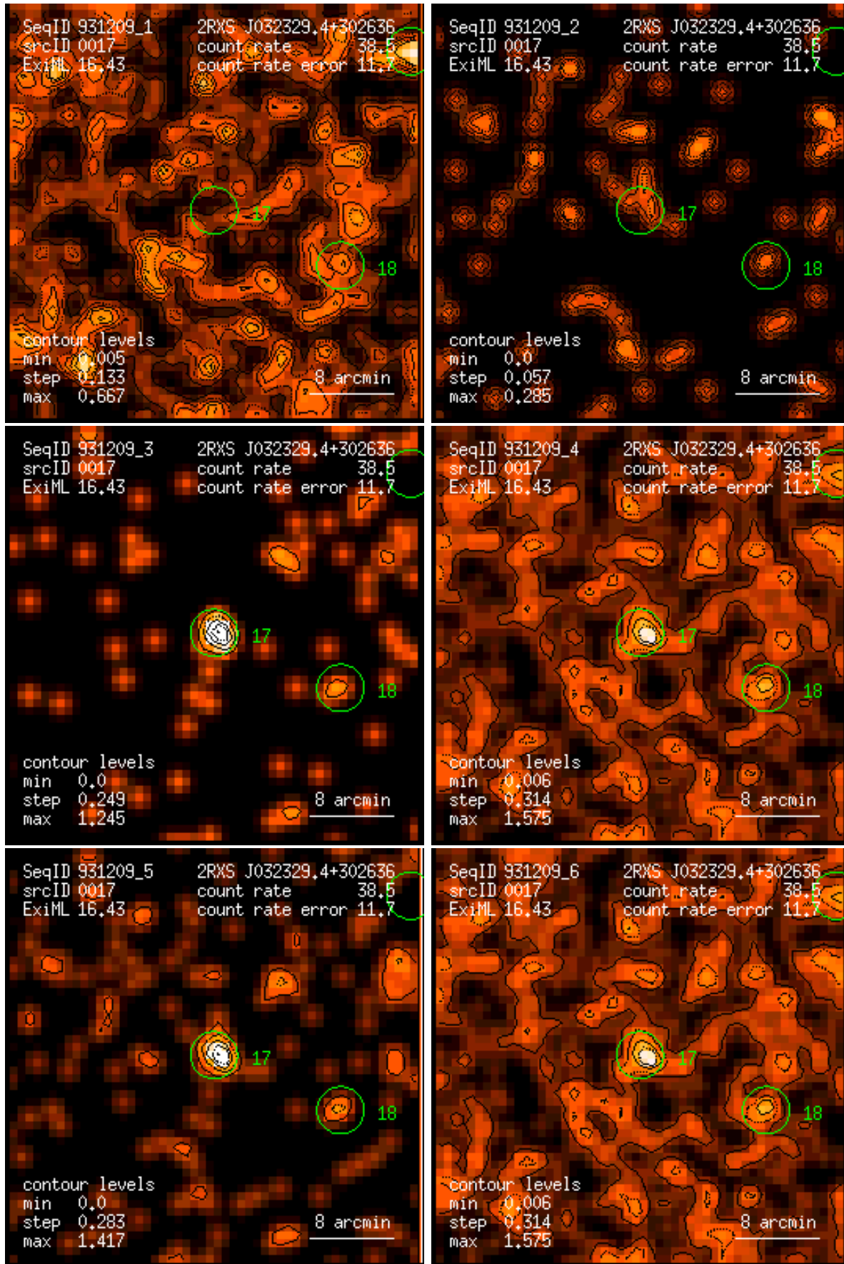
Figure 17: RASS 931209: detection 0017: band rate images, Gaussian filter: (1) PSPC channels 11 – 41, (2) 52 – 90, (3) 91 – 201, (4) 11 – 235, (5) 52 – 201, (6) 11 – 201. Broad band rates in counts/ks. Band rate contour levels in counts/ks/arcmin 2 .
