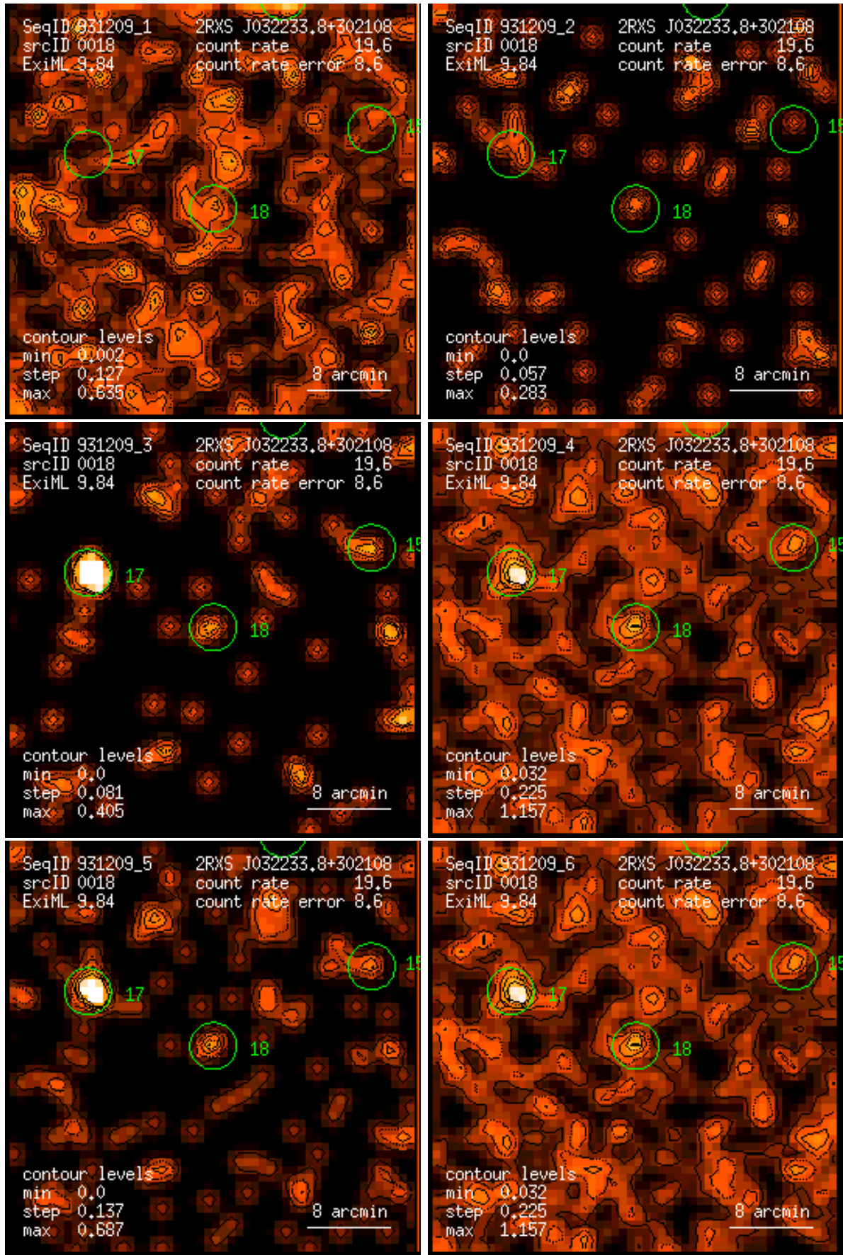
Figure 18: RASS 931209: detection 0018: band rate images, Gaussian filter: (1) PSPC channels 11 – 41, (2) 52 – 90, (3) 91 – 201, (4) 11 – 235, (5) 52 – 201, (6) 11 – 201. Broad band rates in counts/ks. Band rate contour levels in counts/ks/arcmin 2 .
