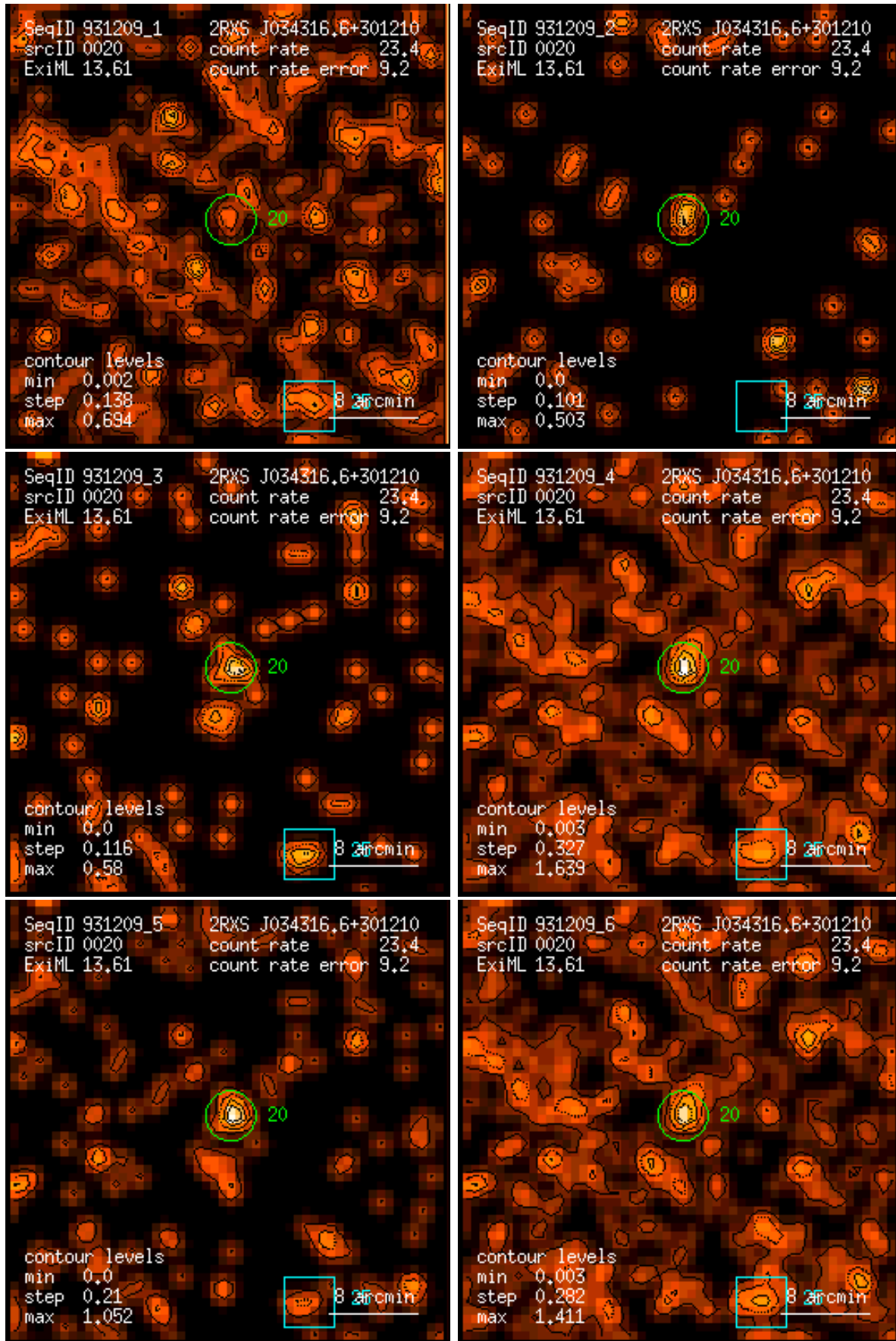
Figure 20: RASS 931209: detection 0020: band rate images, Gaussian filter: (1) PSPC channels 11 – 41, (2) 52 – 90, (3) 91 – 201, (4) 11 – 235, (5) 52 – 201, (6) 11 – 201. Broad band rates in counts/ks. Band rate contour levels in counts/ks/arcmin 2 .
