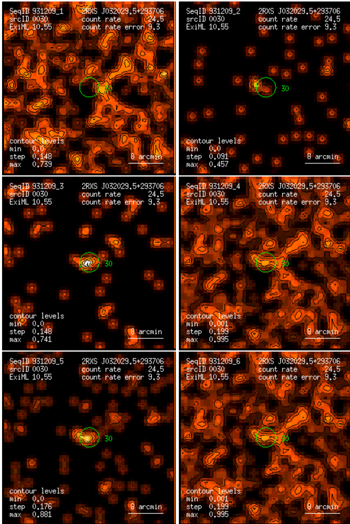
Figure 30: RASS 931209: detection 0030: band rate images, Gaussian filter: (1) PSPC channels 11 – 41, (2) 52 – 90, (3) 91 – 201, (4) 11 – 235, (5) 52 – 201, (6) 11 – 201. Broad band rates in counts/ks. Band rate contour levels in counts/ks/arcmin 2 .
