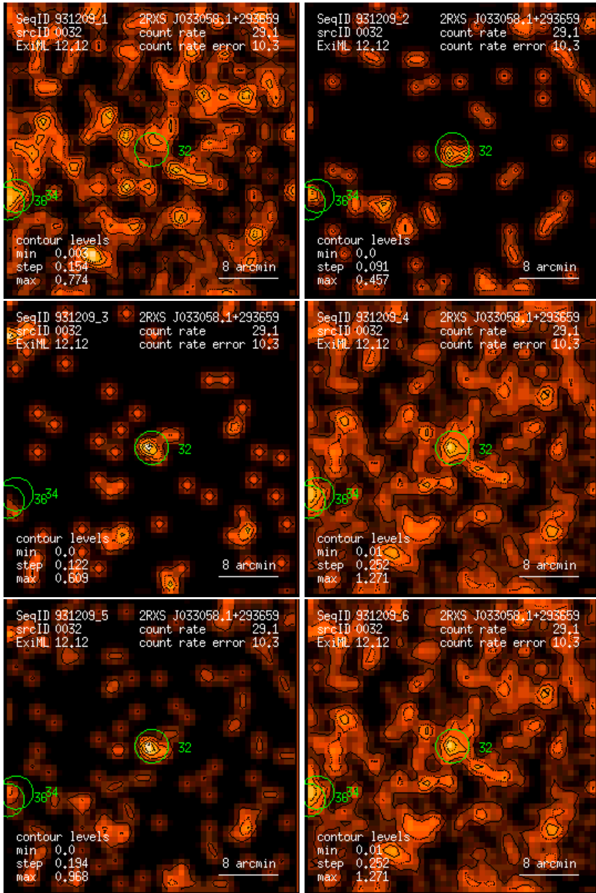
Figure 32: RASS 931209: detection 0032: band rate images, Gaussian filter: (1) PSPC channels 11 – 41, (2) 52 – 90, (3) 91 – 201, (4) 11 – 235, (5) 52 – 201, (6) 11 – 201. Broad band rates in counts/ks. Band rate contour levels in counts/ks/arcmin 2 .
