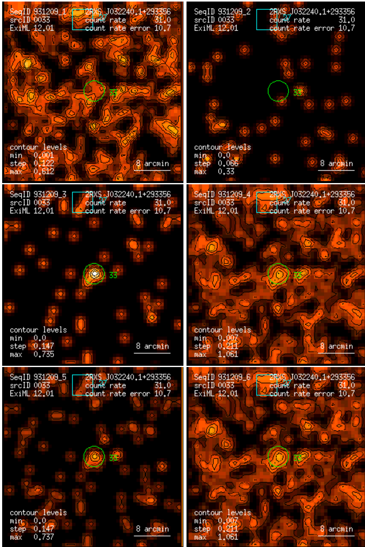
Figure 33: RASS 931209: detection 0033: band rate images, Gaussian filter: (1) PSPC channels 11 – 41, (2) 52 – 90, (3) 91 – 201, (4) 11 – 235, (5) 52 – 201, (6) 11 – 201. Broad band rates in counts/ks. Band rate contour levels in counts/ks/arcmin 2 .
