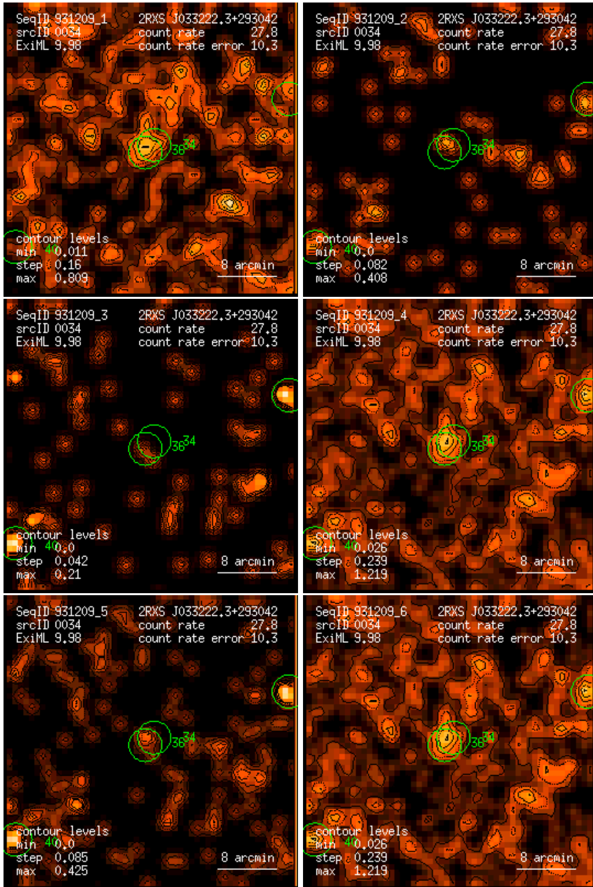
Figure 34: RASS 931209: detection 0034: band rate images, Gaussian filter: (1) PSPC channels 11 – 41, (2) 52 – 90, (3) 91 – 201, (4) 11 – 235, (5) 52 – 201, (6) 11 – 201. Broad band rates in counts/ks. Band rate contour levels in counts/ks/arcmin 2 .
