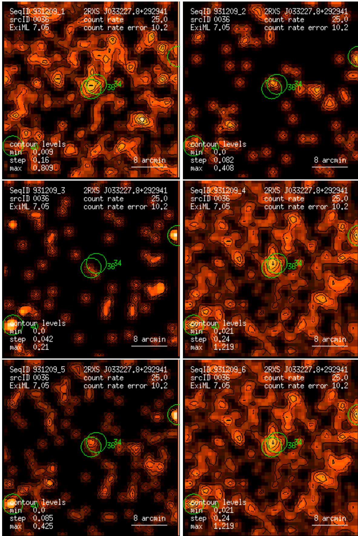
Figure 36: RASS 931209: detection 0036: band rate images, Gaussian filter: (1) PSPC channels 11 – 41, (2) 52 – 90, (3) 91 – 201, (4) 11 – 235, (5) 52 – 201, (6) 11 – 201. Broad band rates in counts/ks. Band rate contour levels in counts/ks/arcmin 2 .
