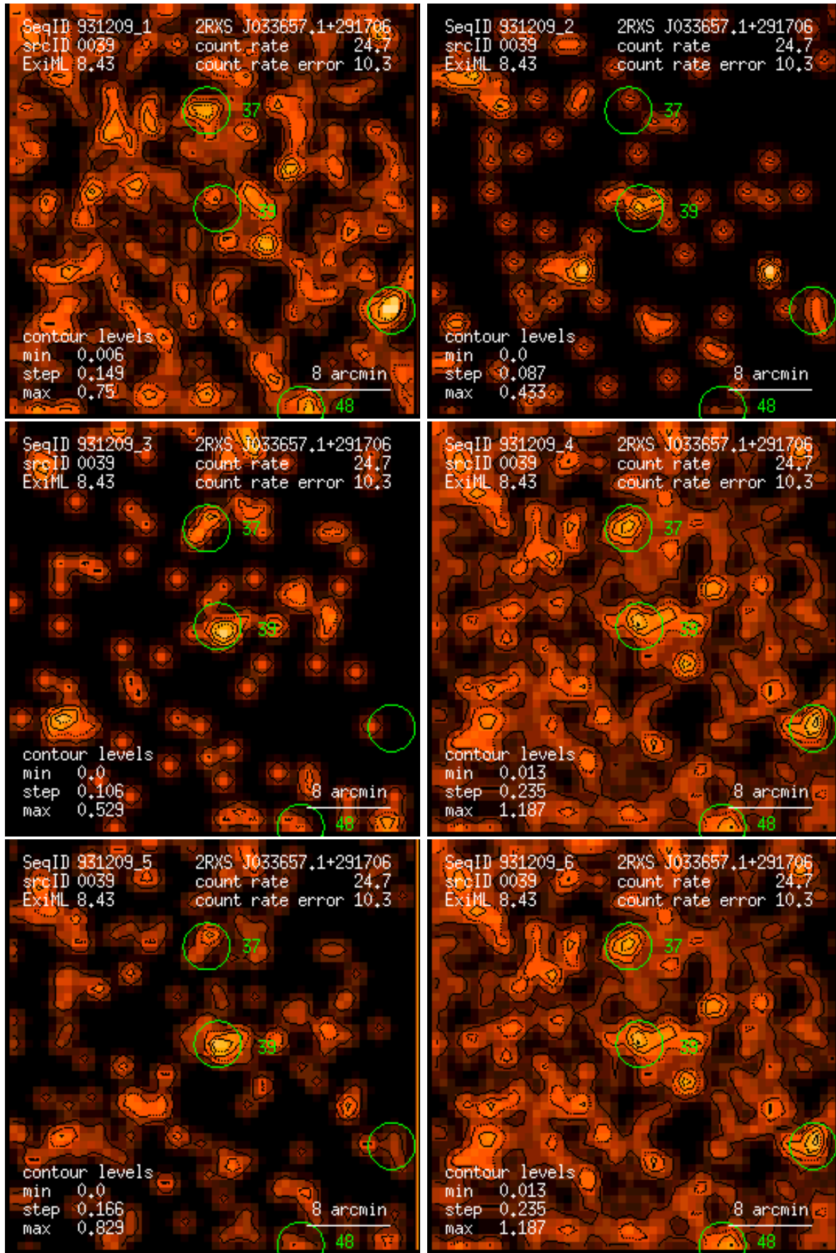
Figure 39: RASS 931209: detection 0039: band rate images, Gaussian filter: (1) PSPC channels 11 – 41, (2) 52 – 90, (3) 91 – 201, (4) 11 – 235, (5) 52 – 201, (6) 11 – 201. Broad band rates in counts/ks. Band rate contour levels in counts/ks/arcmin 2 .
